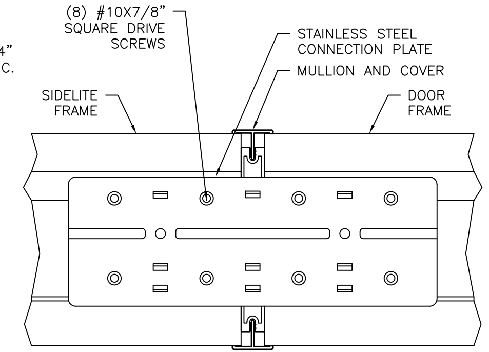
MULLION CONNECTION PLATE INSTALLATION DETAIL AT HEAD AND SILL
