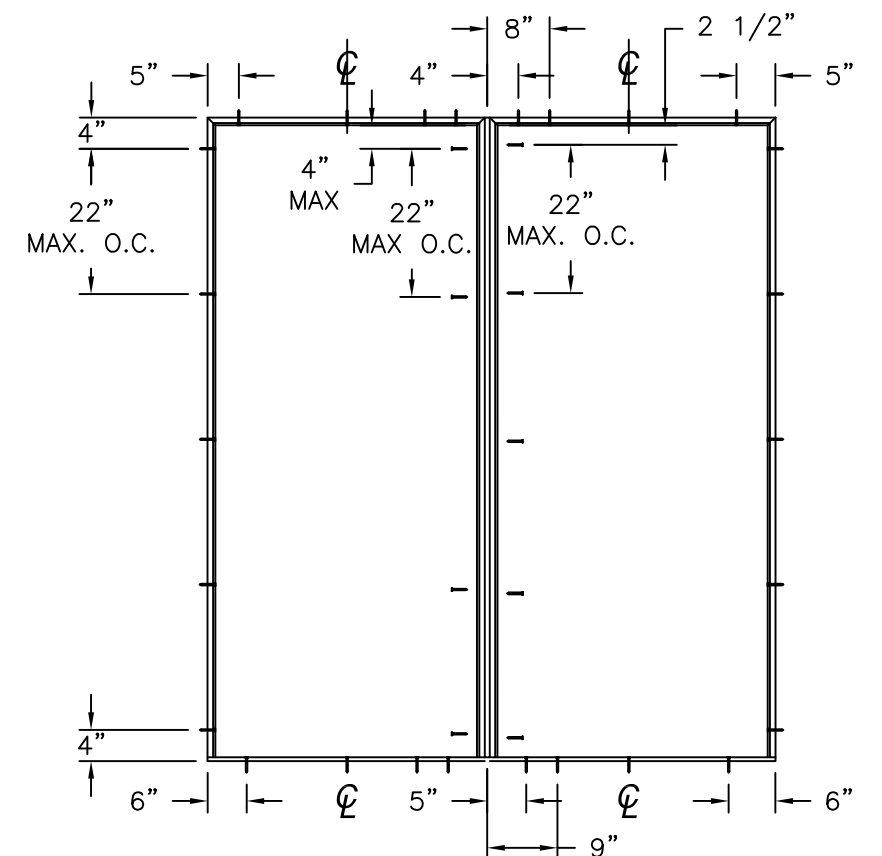
ANCHORING LAYOUT FOR OX AND XO (MULL)
