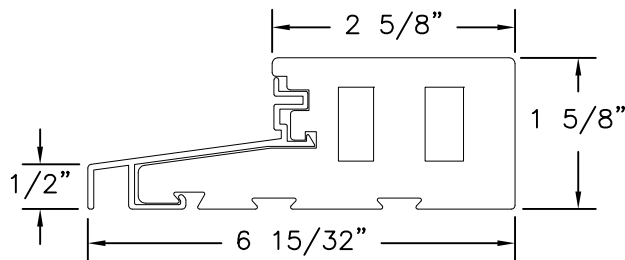
OUTSWING DOOR SILL DETAIL
