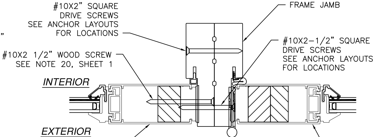
MULLION DETAIL
