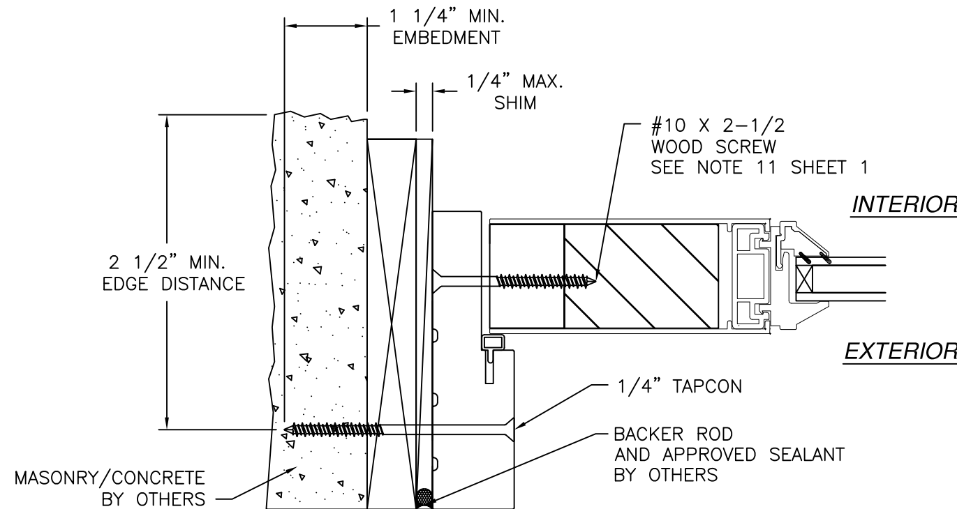
SIDELITE JAMB INSTALLATION DETAIL MASONRY/CONCRETE
