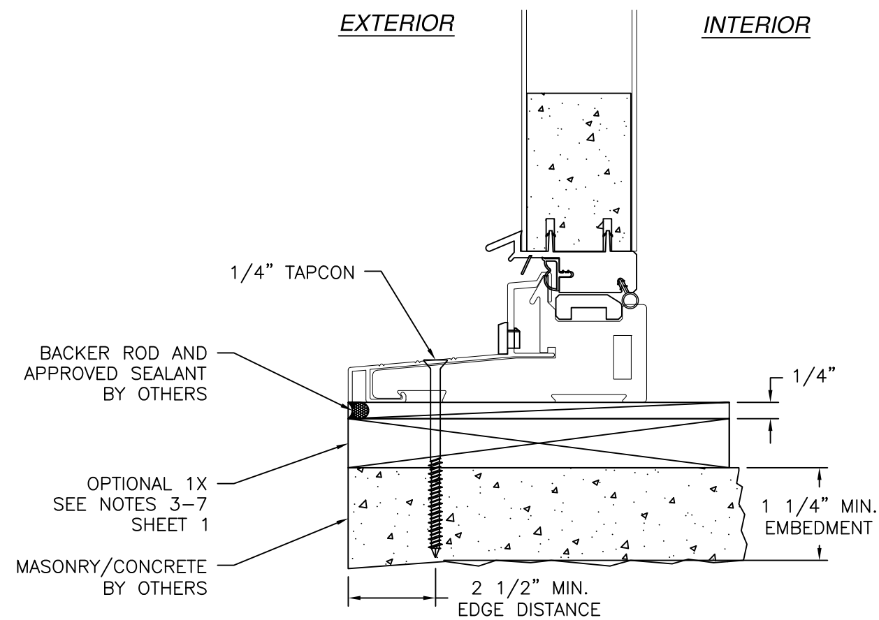
SIDELITE INSTALLATION DETAIL MASONRY/CONCRETE
