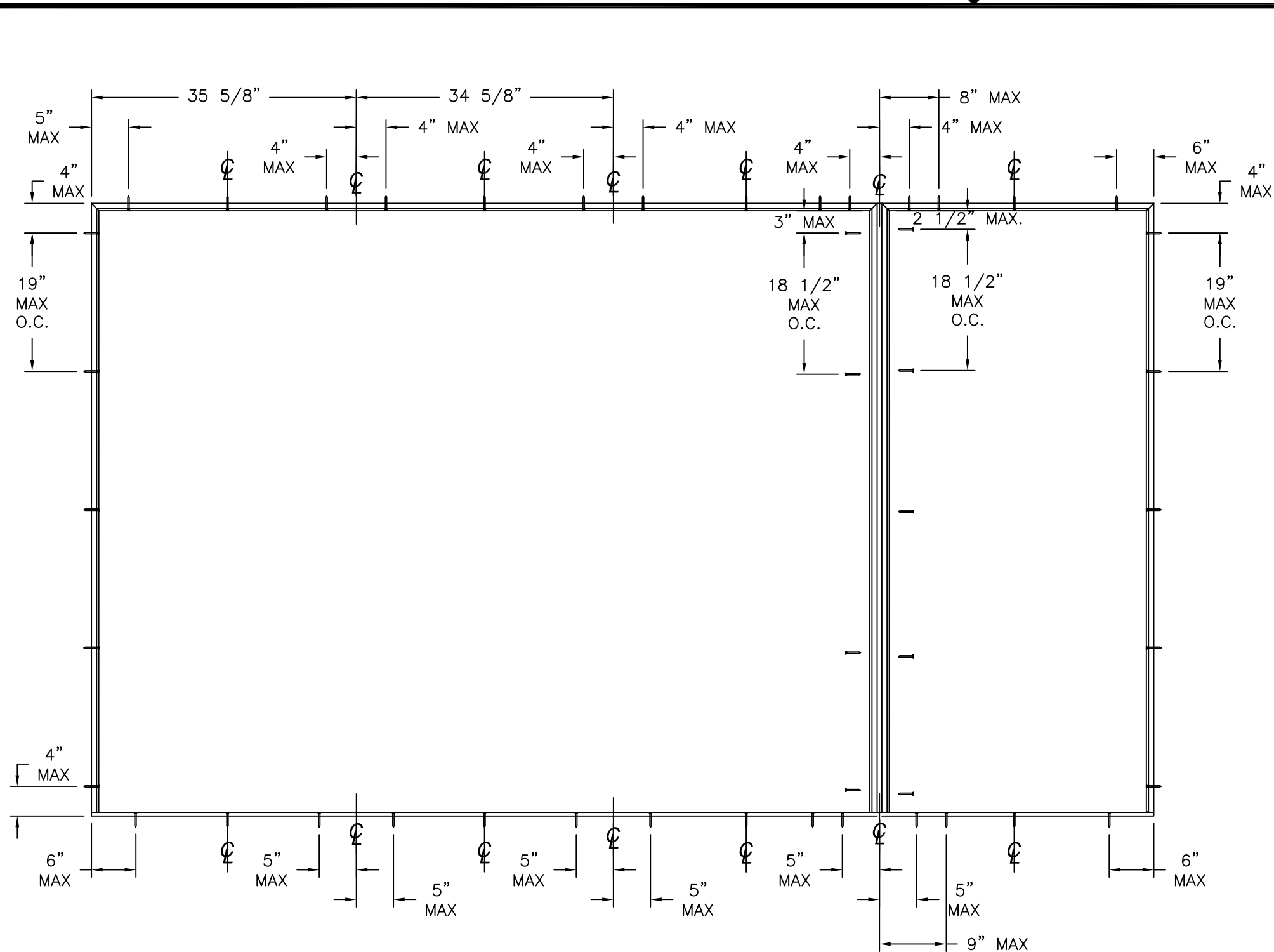
ANCHORING LAYOUT
