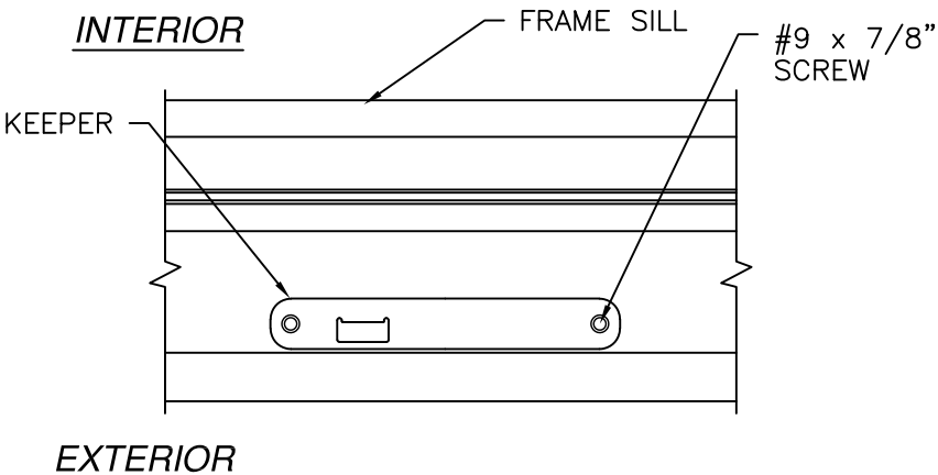
SILL KEEPER DETAIL
