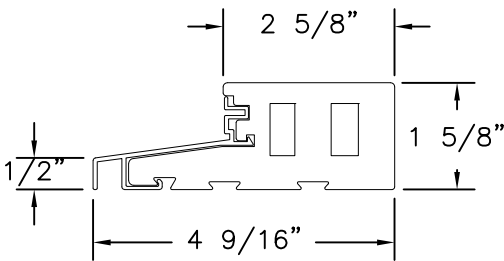
OUTSWING DOOR SILL DETAIL
