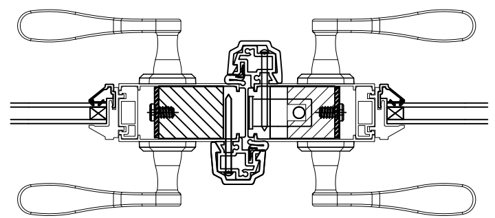
LOCKING SYSTEM DETAIL
