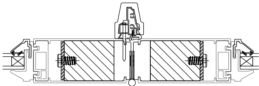
HINGE DETAIL
