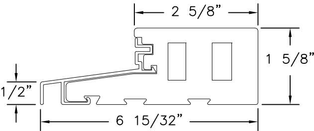
OUTSWING DOOR SILL DETAIL
