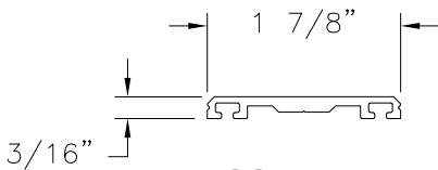
PRESSURE PLATE ALUMINUM (S34792)
