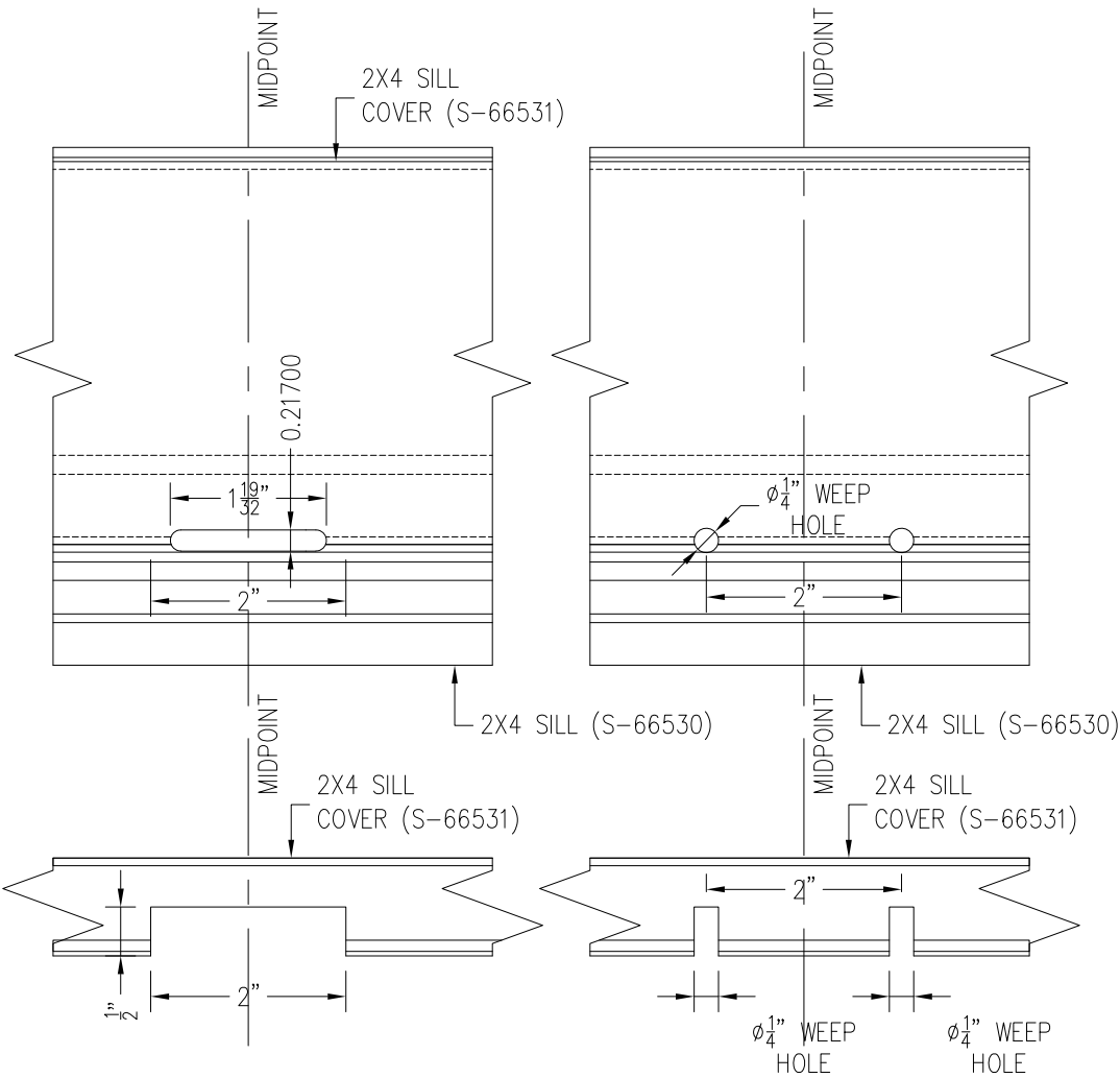
WEEP HOLE DETAIL @ CENTER OF BAY
