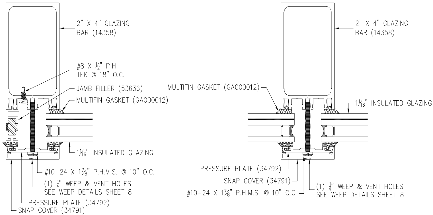
HORIZONTAL CROSS SECTION
