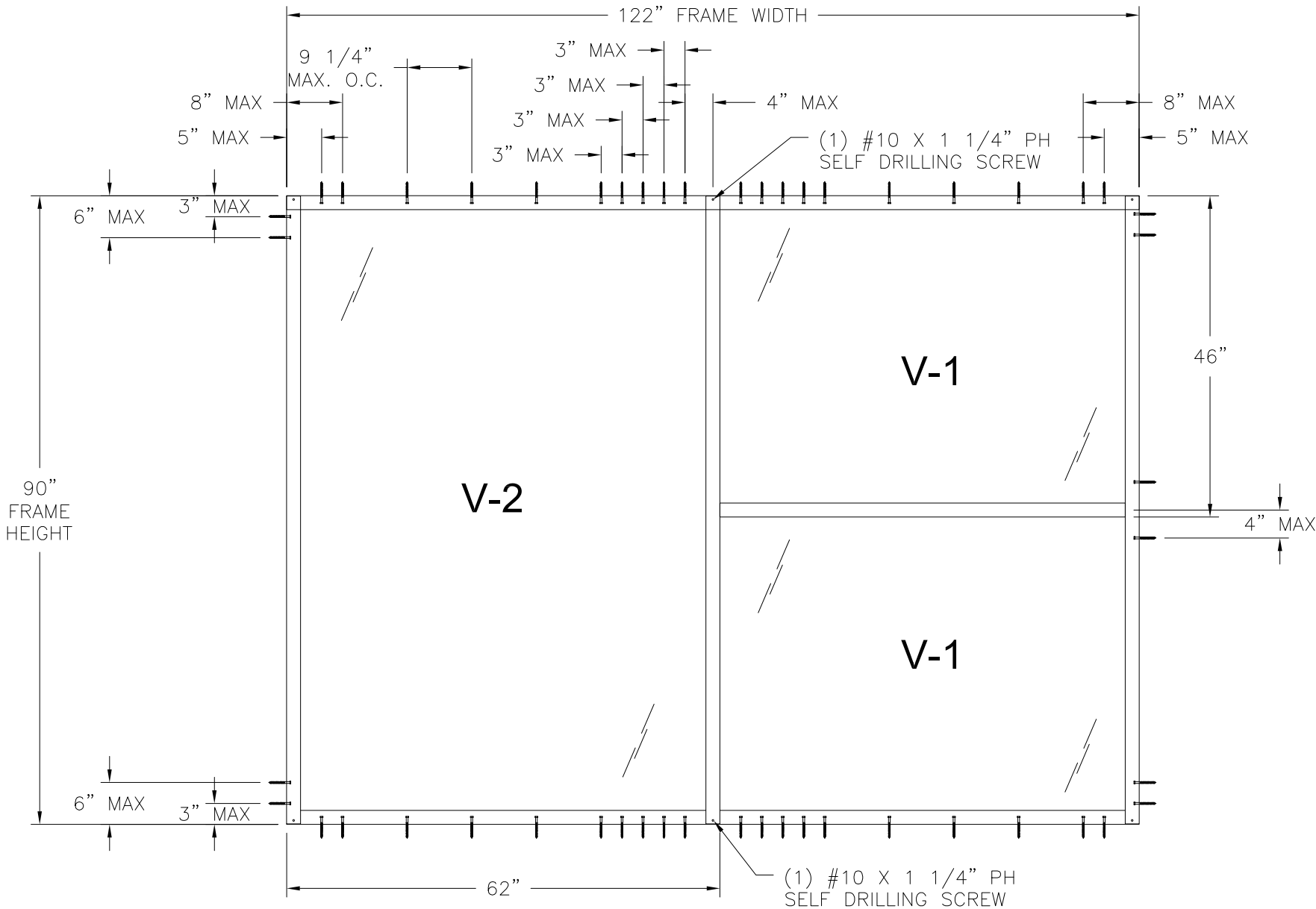
SI5008 ALUMINUM FIXED CURTAIN WALL WITH 1/4" LAG SCREWS, 1/4" SMS OR SELF DRILLING SCREWS AND 1/4" ELCO ULTRACON EXTERIOR VIEW
