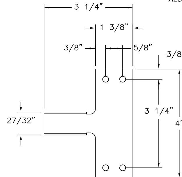
MT000022 CLIP 16GA (.063") GALVANIZED STEEL
