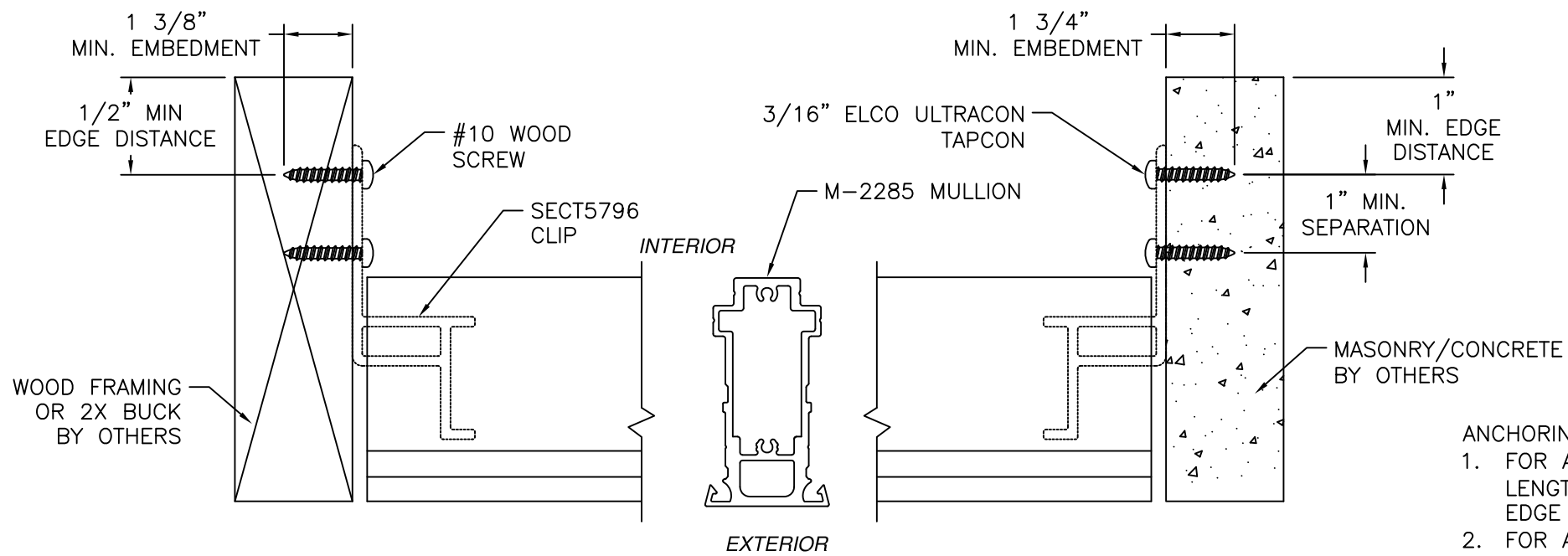
MULLION INSTALLATION WOOD & CONCRETE
