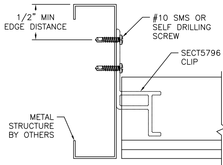
MULLION INSTALLATION METAL
