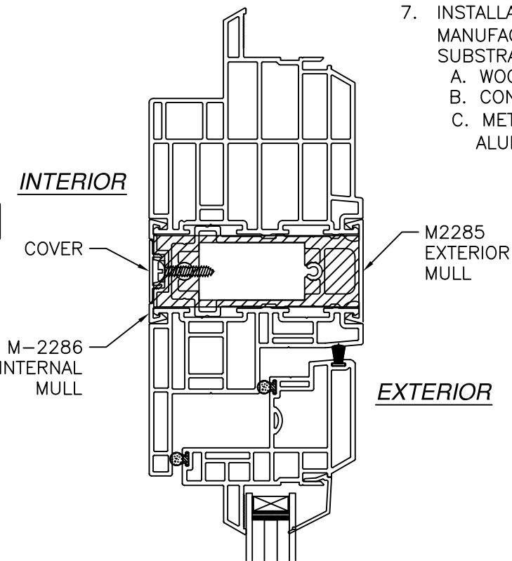
WINDOW & MULLION ASSEMBLY REFERENCE ONLY
