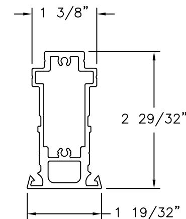
M-2285 MULLION ALUMINUM 6005-T5 .125" THICK
