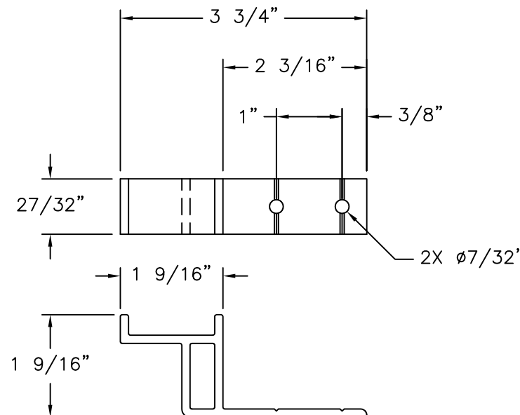
SECT5796 CLIP FOR WOOD FRAMING INSTALLATION ALUMINUM 6063-T5 .125" THICK
