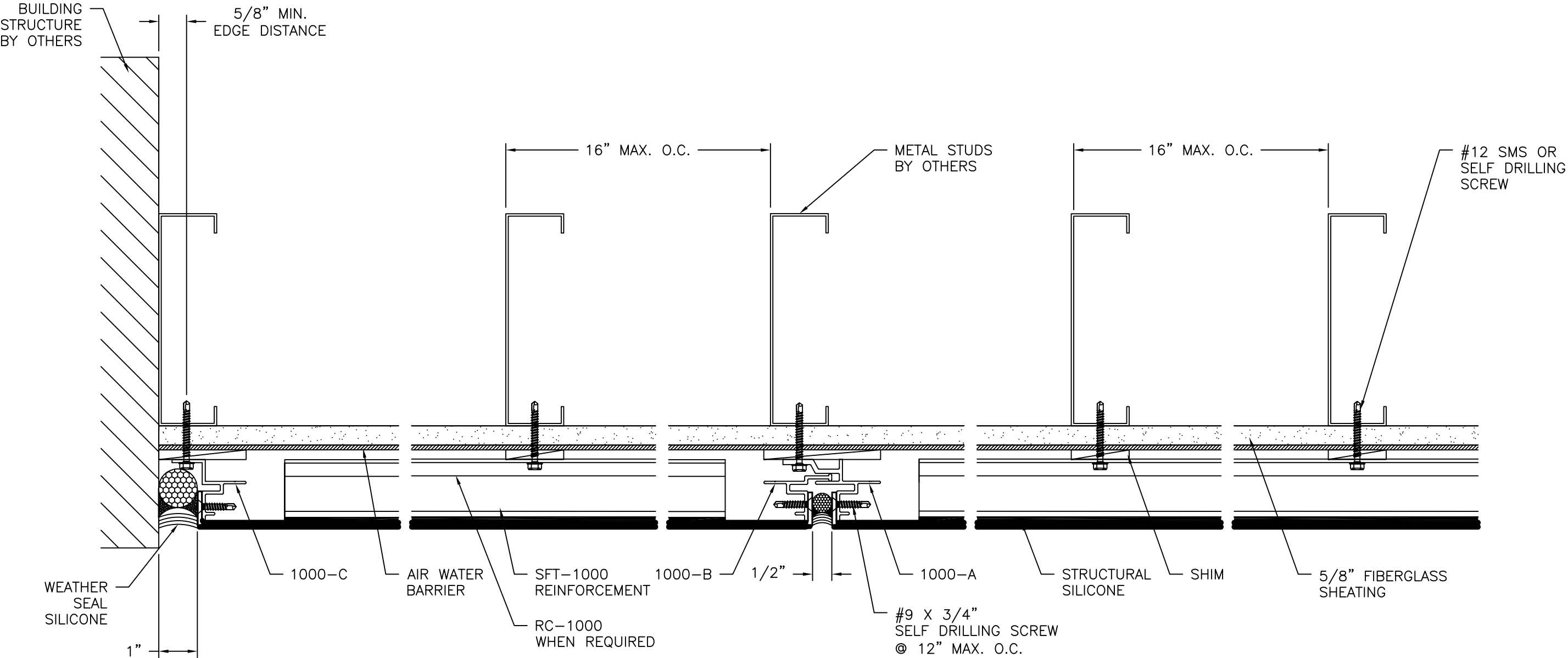
C 5 HORIZONTAL CROSS SECTION
