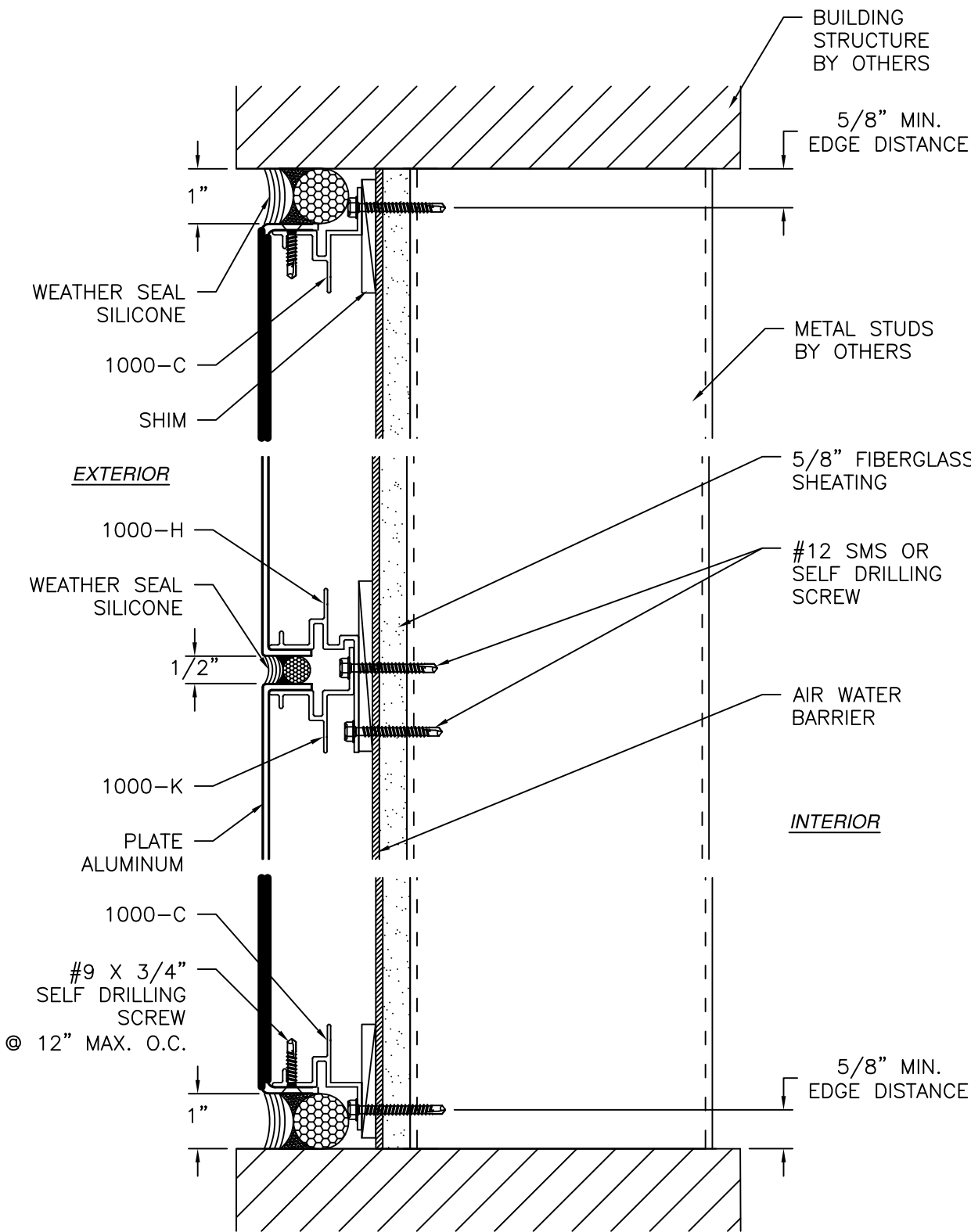
B 4 VERTICAL CROSS SECTION
