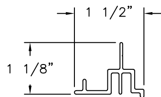
1000-PJ ALUMINUM 6005A-T6 (.080" THICK)
