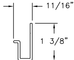
ET-J ALUMINUM 6063-T6 (.080" THICK)
