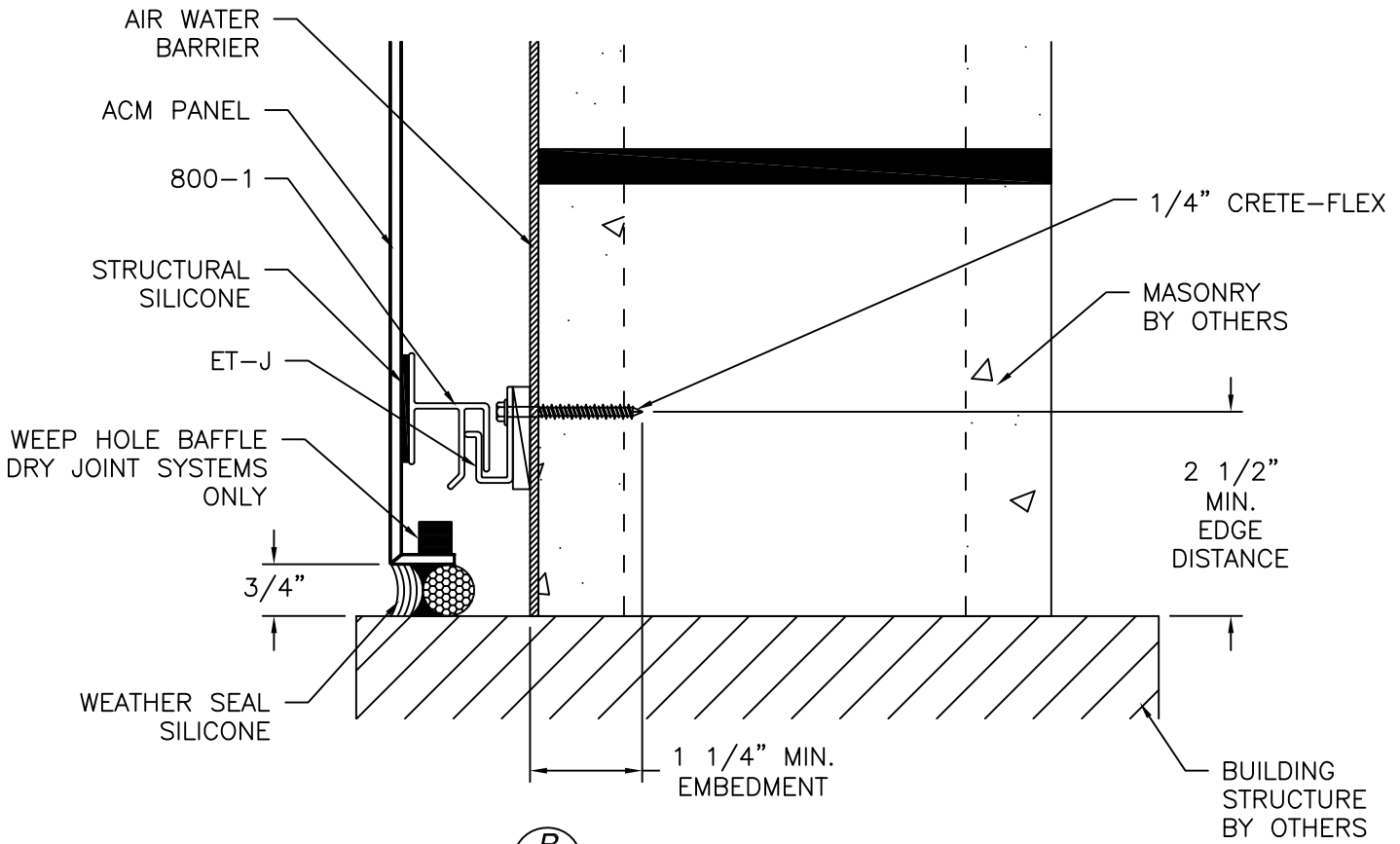
B 3 VERTICAL CROSS SECTION
