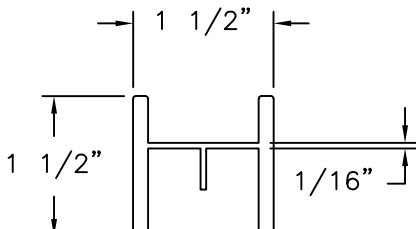
STF-1000 ALUMINUM 6063-T6 (.160" THICK)
