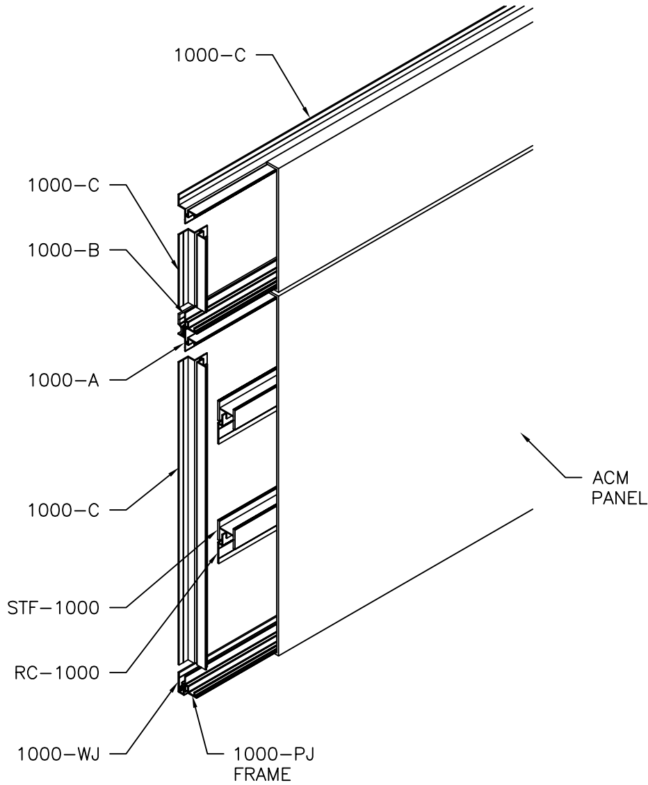
INSTALLATION DETAIL
