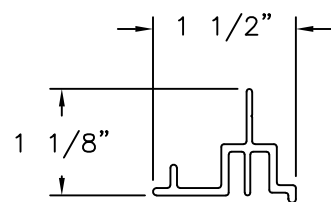
1000-PJ ALUMINUM 6005A-T6 (.080" THICK)
