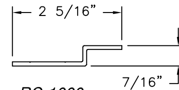
RC-1000 ALUMINUM 6063-T6 (.125" THICK)
