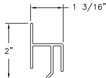
800-1 ALUMINUM 6063-T6 (.080" THICK)
