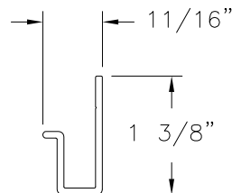
ET-J ALUMINUM 6063-T6 (.080" THICK)
