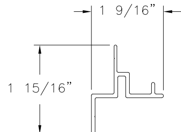
1000-K ALUMINUM 6005A-T6 (.080" THICK)
