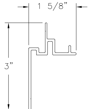
1000-H ALUMINUM 6005A-T6 (.080" THICK)
