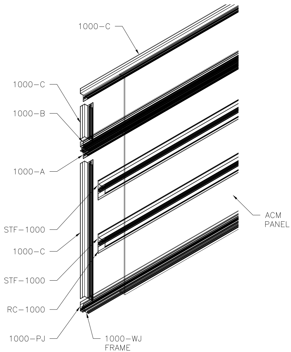
INSTALLATION DETAIL
