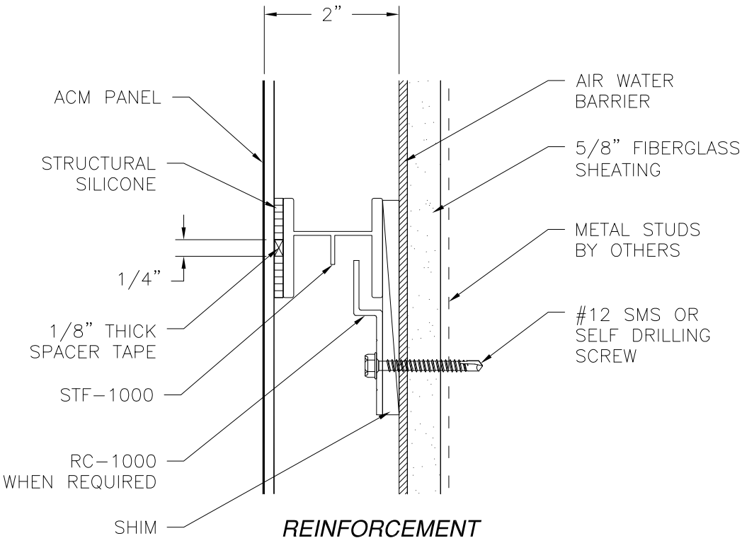
REINFORCEMENT INSTALLATION DETAIL
