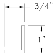
ET-Q ALUMINUM 6063-T6 (.125" THICK)
