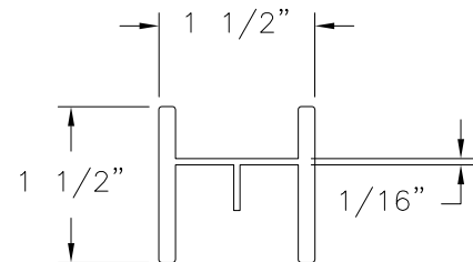
STF-1000 ALUMINUM 6063-T6 (.160" THICK)
