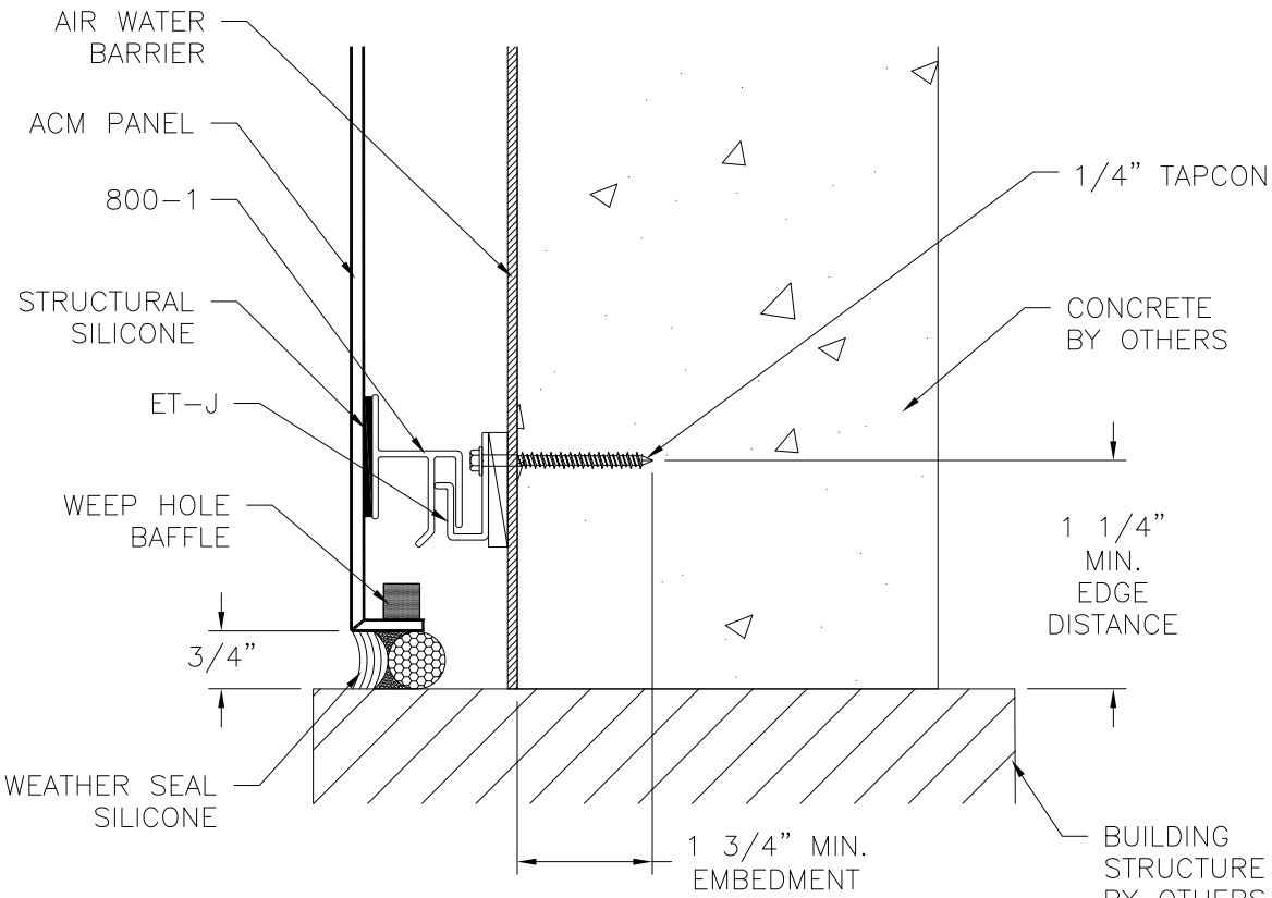
B 3 VERTICAL CROSS SECTION
