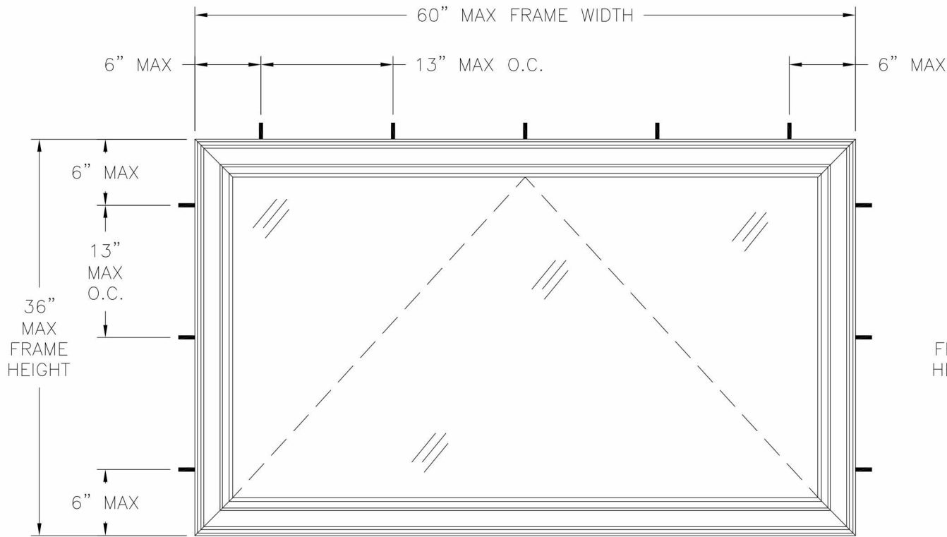
9660 AWNING WINDOW EXTERIOR VIEW FINLESS & FLANGE INSTALLATION
