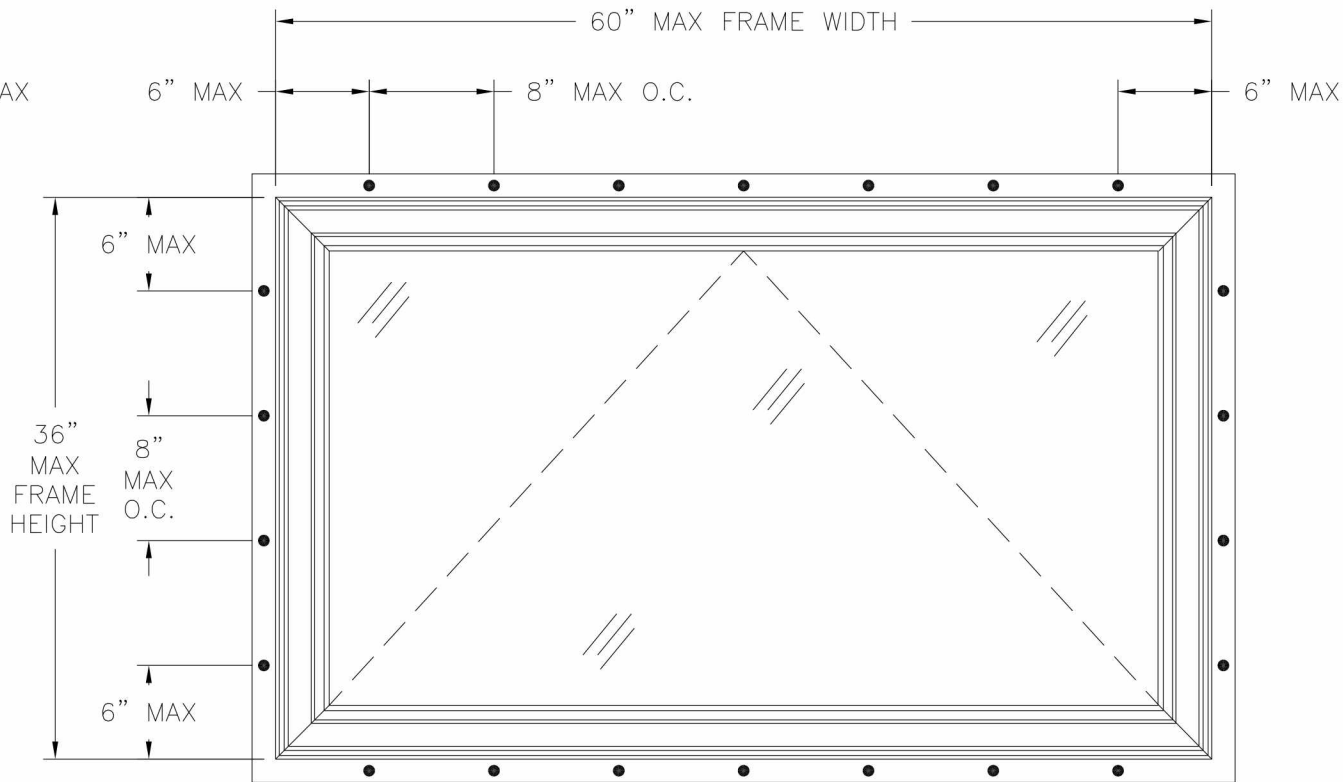
9660 AWNING WINDOW EXTERIOR VIEW FIN INSTALLATION
