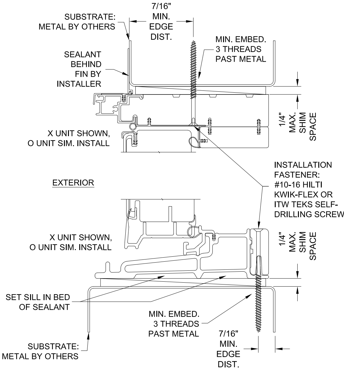
TYPICAL FRAME VERTICAL SECTION
