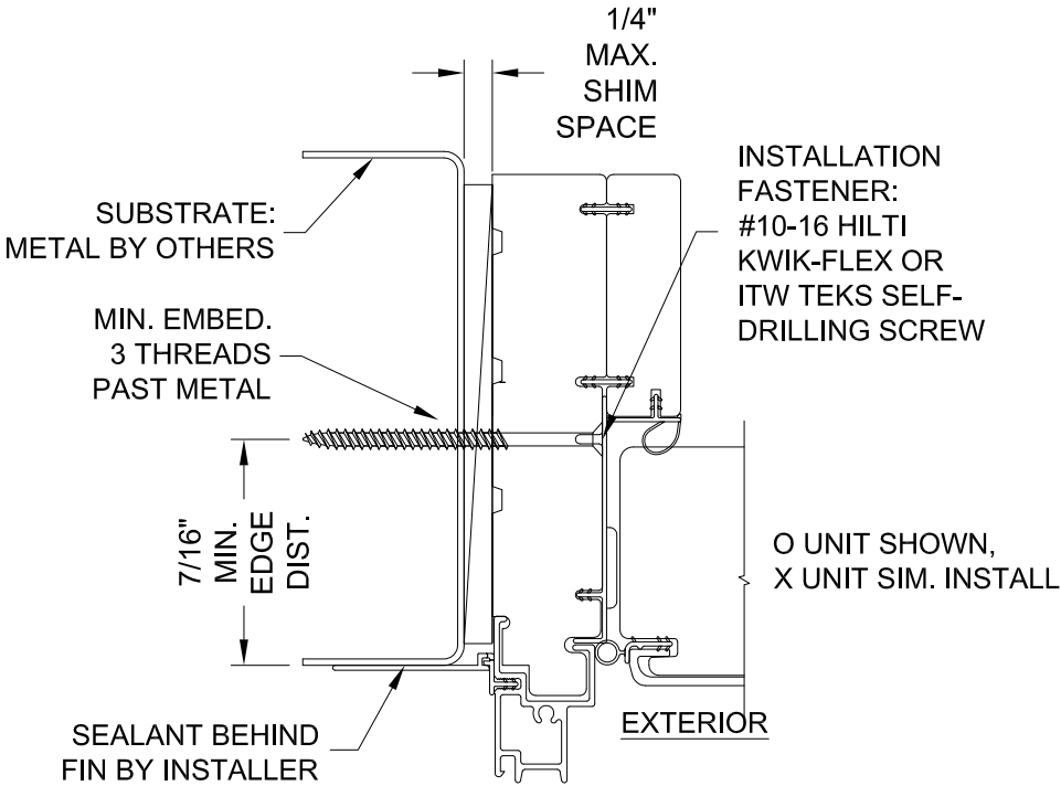
TYPICAL JAMB HORIZONTAL SECTION
