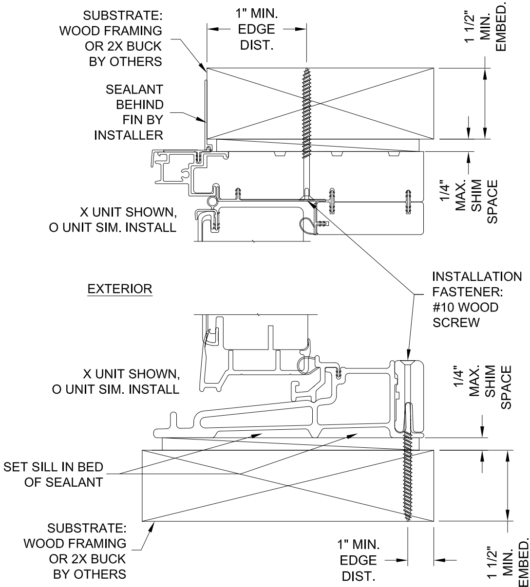
TYPICAL FRAME VERTICAL SECTION
