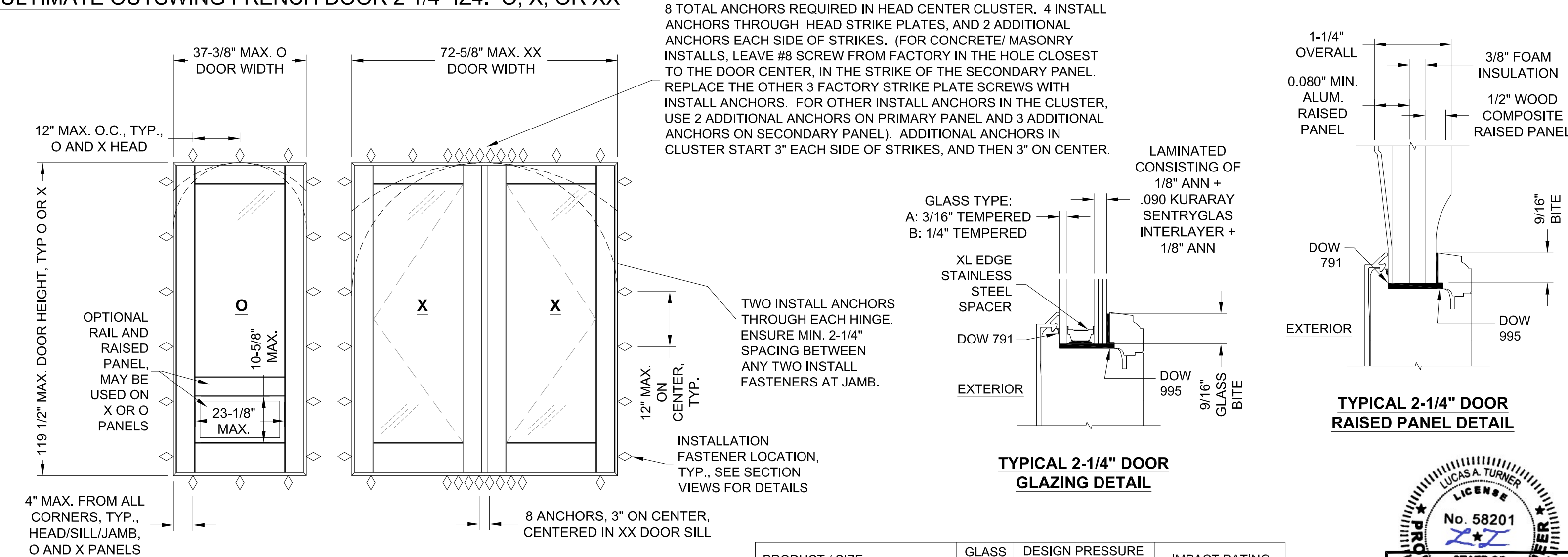
TYPICAL ELEVATIONS RECTANGULAR TOP, RADIUS TOP, AND ARCH TOP ALLOWED
