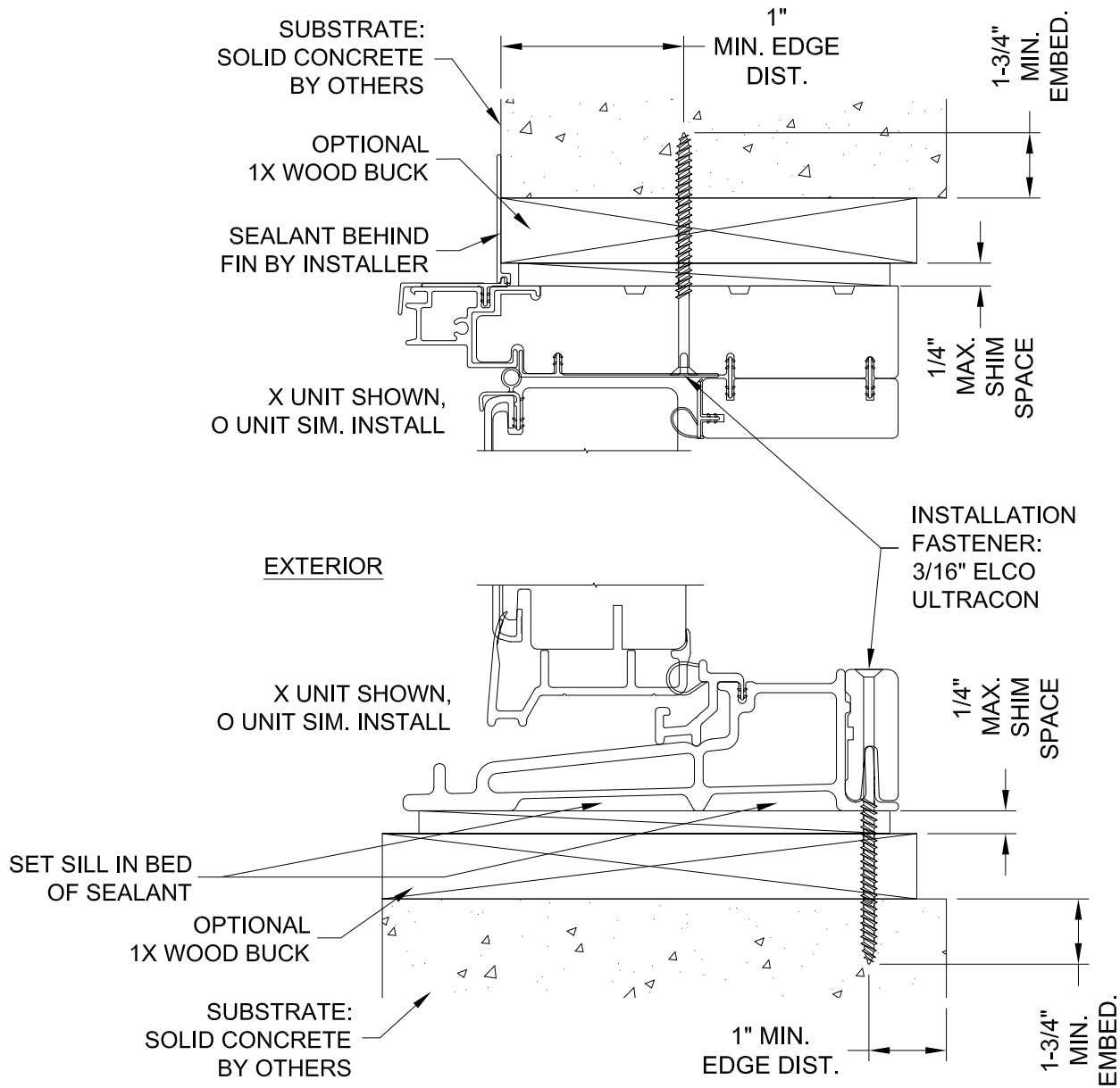
TYPICAL FRAME VERTICAL SECTION
