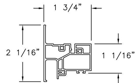
FIXED MEETING RAIL PVC
