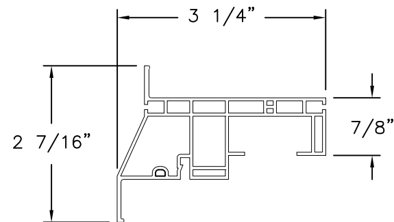
HEAD, SILL AND JAMB PVC
