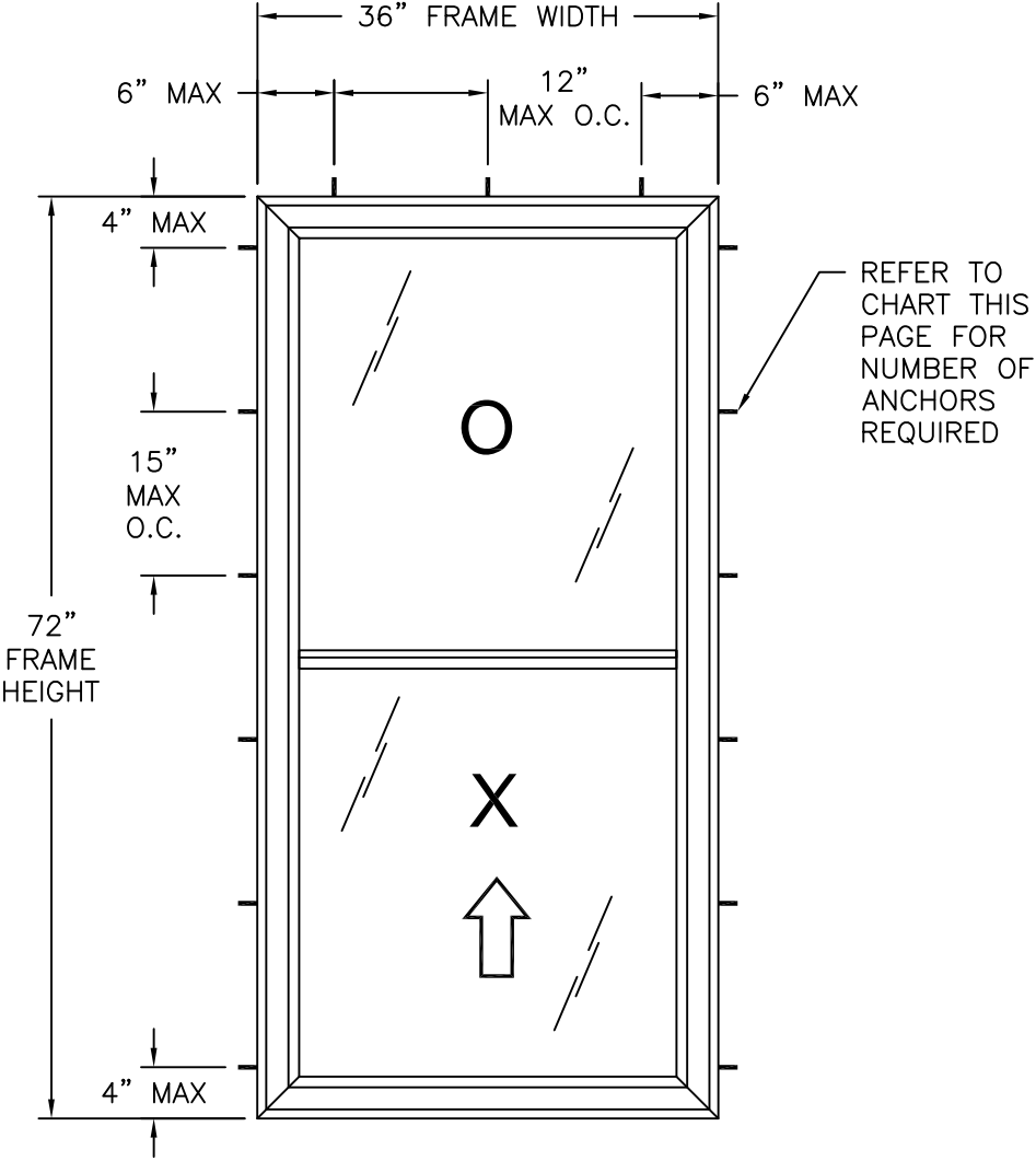
SERIES 3500 HP FLANGE PVC SINGLE HUNG WINDOW EXTERIOR VIEW
