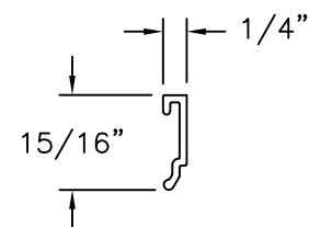
GLAZING BEAD PVC
