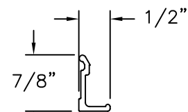
LIFT BEAD PVC
