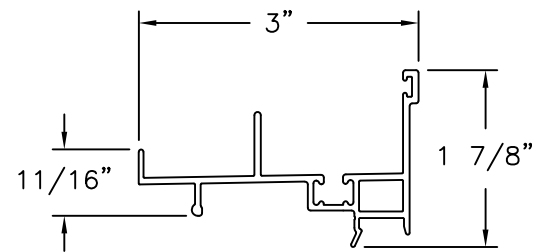
SNAP IN SILL PVC
