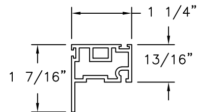
SASH RAIL PVC
