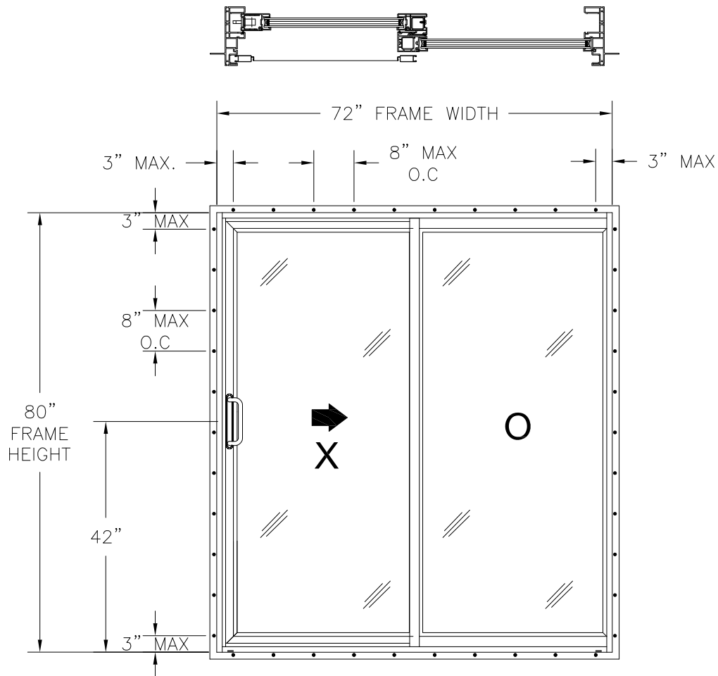
SERIES 910/3910 PVC SLIDING GLASS DOOR
