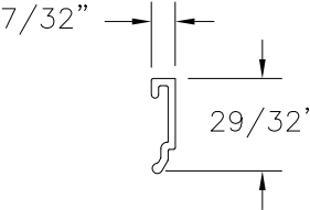
GLAZING BEAD RIGID PVC .070" THICKNESS (V-782)
