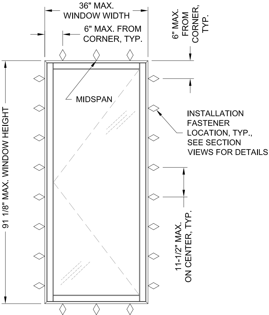
TYPICAL ELEVATION
