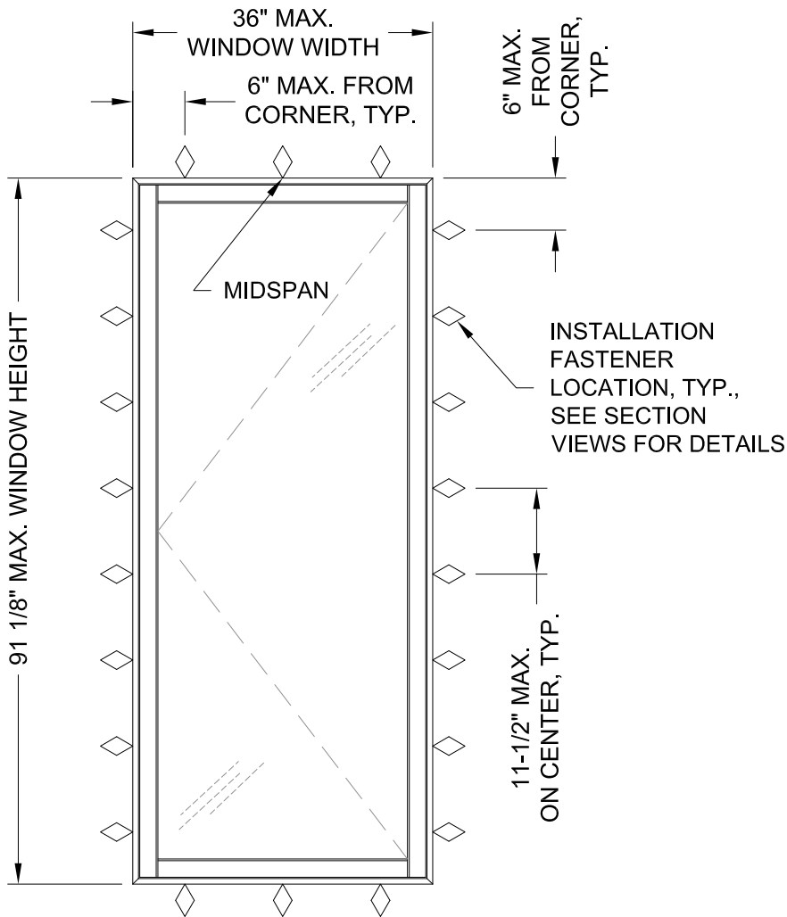
TYPICAL ELEVATION
