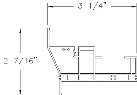
MAIN FRAME W/FLANGE EXTRUDED RIGID PVC
