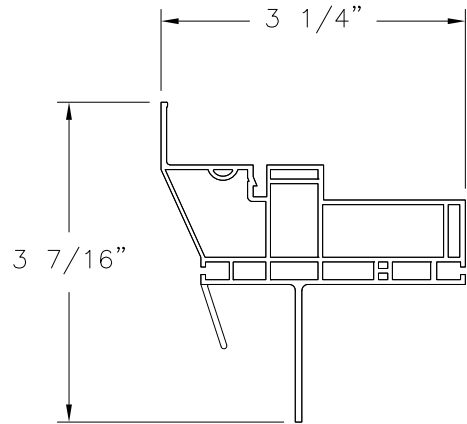
MAIN FRAME FIN INSTALLATION W/J-CHANNEL EXTRUDED RIGID PVC
