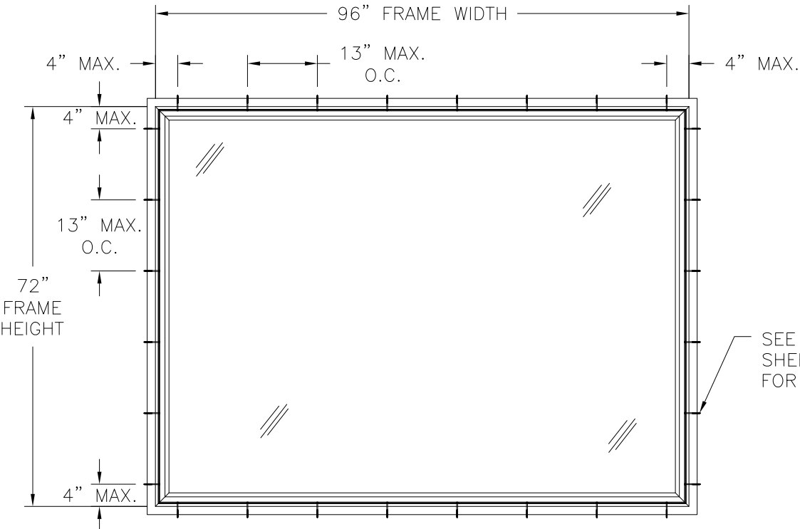
SERIES 3500 HP, 3500 HPPW, 3500 HPSDLITES, 3500 HPSP, 3500 HPT, 1255 HPPW PVC FIXED WINDOW FLANGE INSTALLATION
