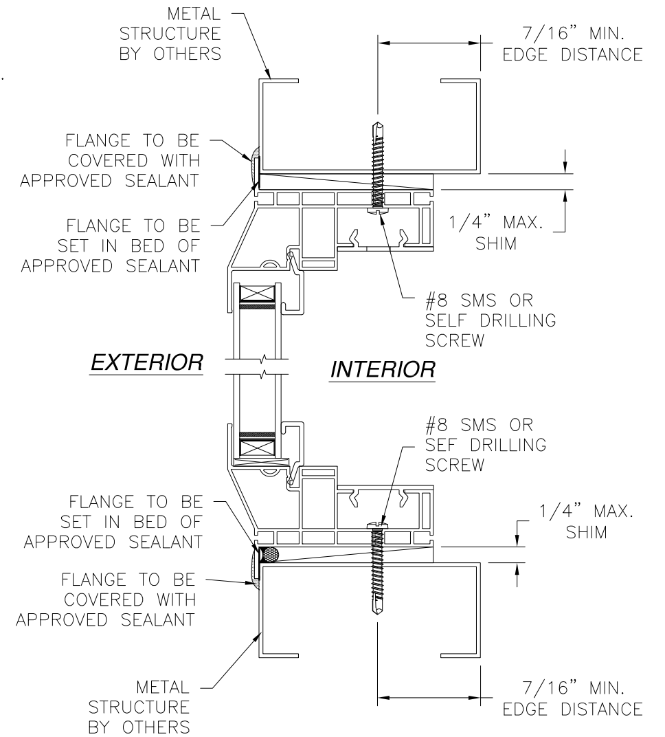
VERTICAL CROSS SECTION 2X BUCK/WOOD FLANGE INSTALLATION HEAD AND SILL SHOWN, JAMBS SIMILAR
