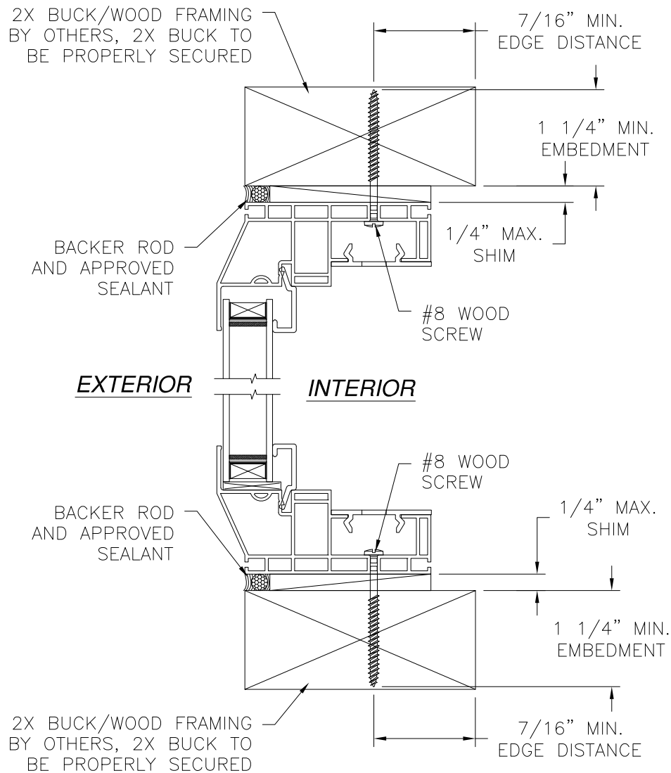
VERTICAL CROSS SECTION 2X BUCK/WOOD FLUSH INSTALLATION HEAD AND SILL SHOWN, JAMBS SIMILAR
