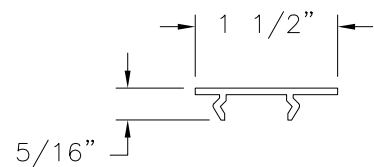
MAIN FRAME COVER EXTRUDED RIGID PVC
