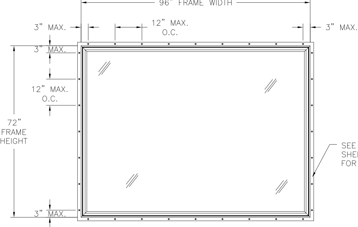
SERIES 3500 HP, 3500 HPPW, 3500 HPSDLITES, 3500 HPSP, 3500 HPT, 1255 HPPW PVC FIXED WINDOW FIN INSTALLATION
