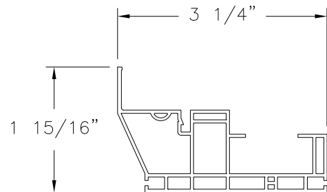
MAIN FRAME EXTRUDED RIGID PVC
