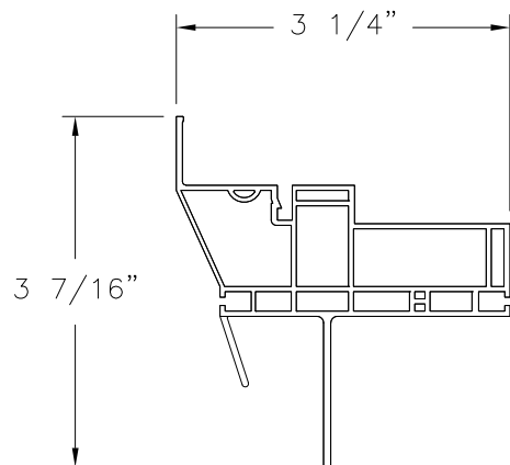
MAIN FRAME FIN INSTALLATION EXTRUDED RIGID PVC
