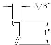
GLAZING BEAD EXTRUDED RIGID PVC
