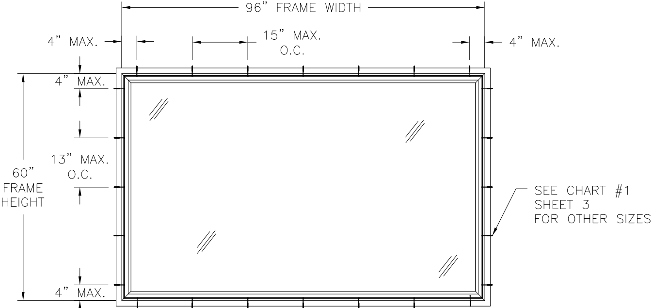
SERIES 3500 HP, 3500 HPPW, 3500 HPSDLITES, 3500 HPSP, 3500 HPT, 1255 HPPW PVC FIXED WINDOW FLANGE INSTALLATION
