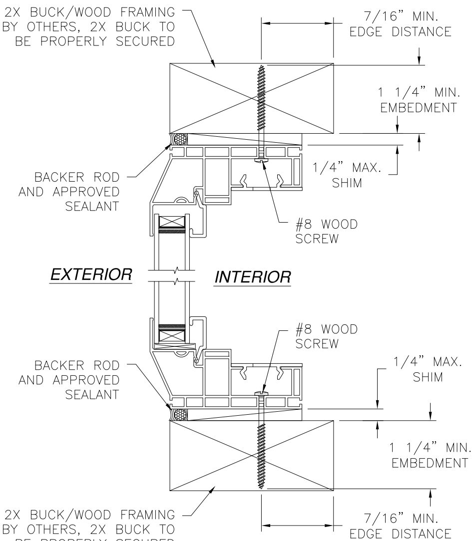
VERTICAL CROSS SECTION 2X BUCK/WOOD INSTALLATION HEAD AND SILL SHOWN, JAMBS SIMILAR
