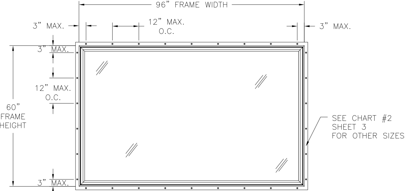
SERIES 3500 HP, 3500 HPPW, 3500 HPSDLITES, 3500 HPSP, 3500 HPT, 1255 HPPW PVC FIXED WINDOW FIN INSTALLATION
