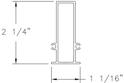
REINFORCEMENT (2480-A) ALUMINUM 6063-T5
