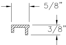
REINFORCEMENT (2244-A) ALUMINUM 6063-T5
