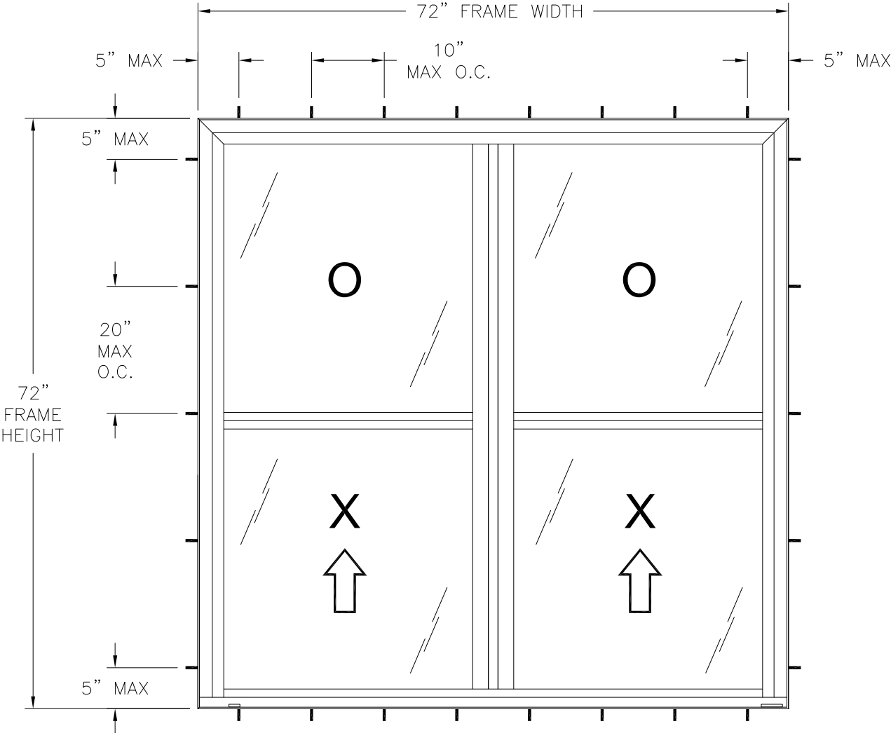
SERIES 450 TWIN CHS SINGLE HUNG WINDOW EXTERIOR VIEW
