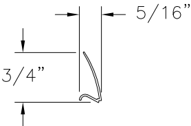
GLAZING BEAD (1718R) EXTRUDED RIGID PVC
