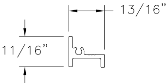
REINFORCEMENT (2230-C) ALUMINUM 6063-T5
