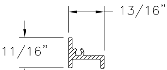
REINFORCEMENT (S-046) ALUMINUM 6061-T6
