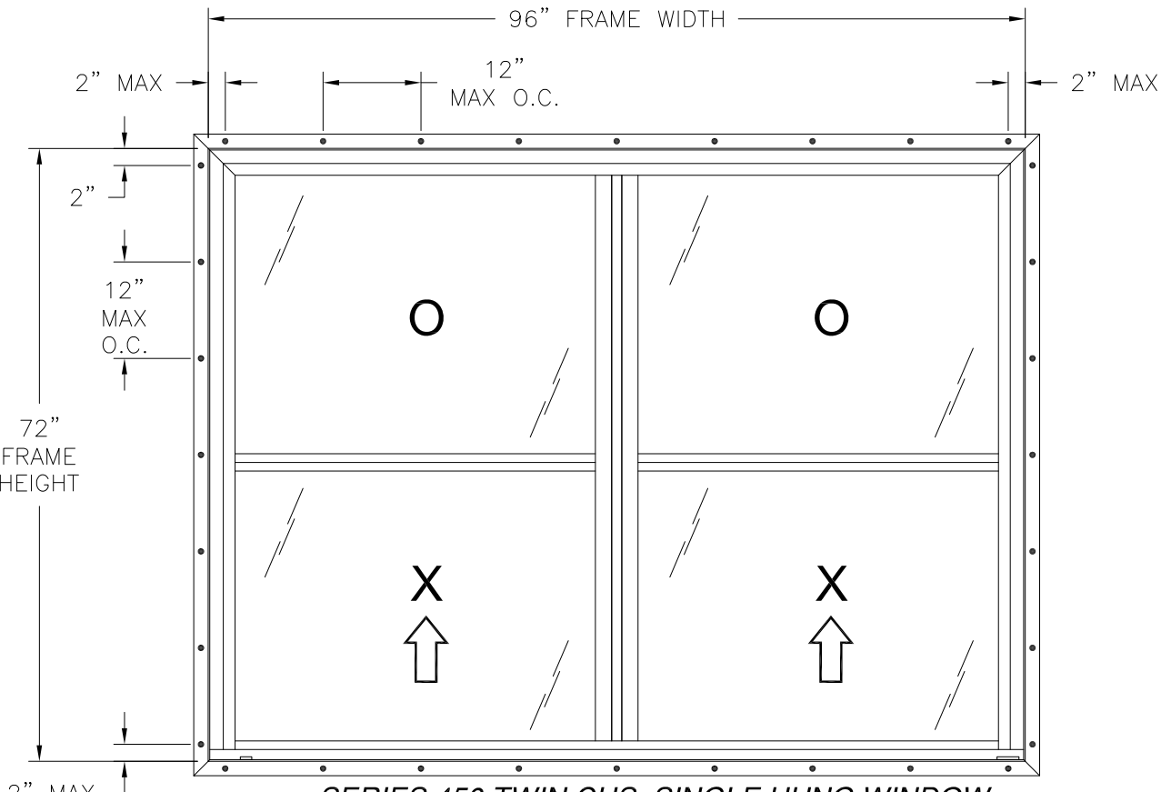
SERIES 450 TWIN CHS SINGLE HUNG WINDOW EXTERIOR VIEW FIN INSTALLATION
