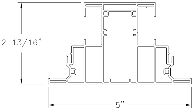
INTERMEDIATE MULLION (V-718) EXTRUDED RIGID PVC
