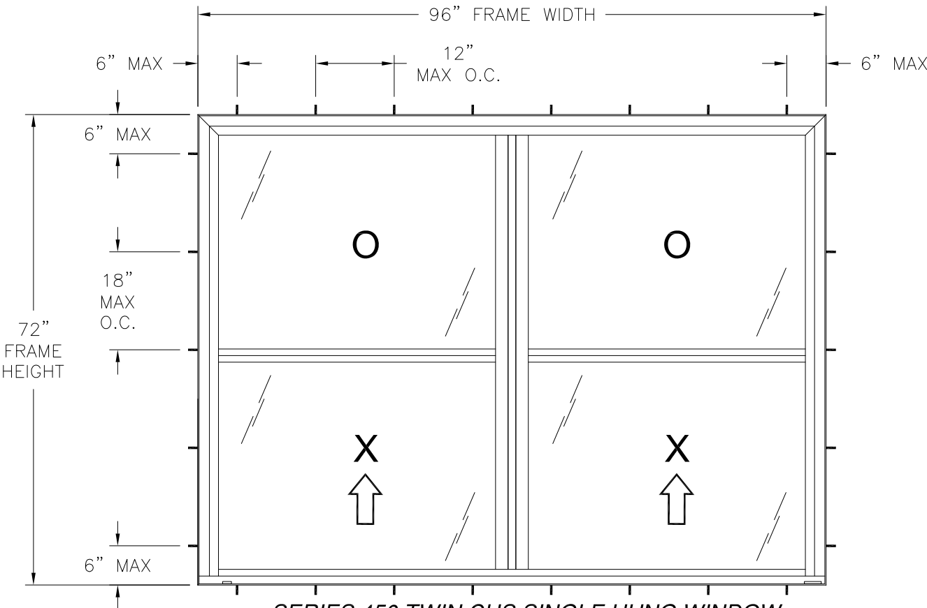
SERIES 450 TWIN CHS SINGLE HUNG WINDOW EXTERIOR VIEW FRAME INSTALLATION
