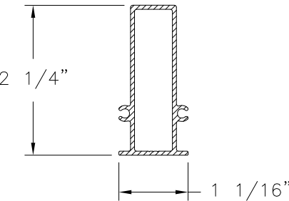
REINFORCEMENT ALUMINUM 6063-T5
