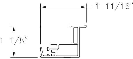
SASH LOCK RAIL (V-704) EXTRUDED RIGID PVC
