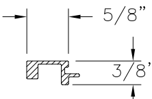
REINFORCEMENT (S-047) ALUMINUM 6061-T6
