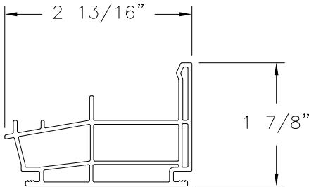
SILL FRAME (V-871) EXTRUDED RIGID PVC
