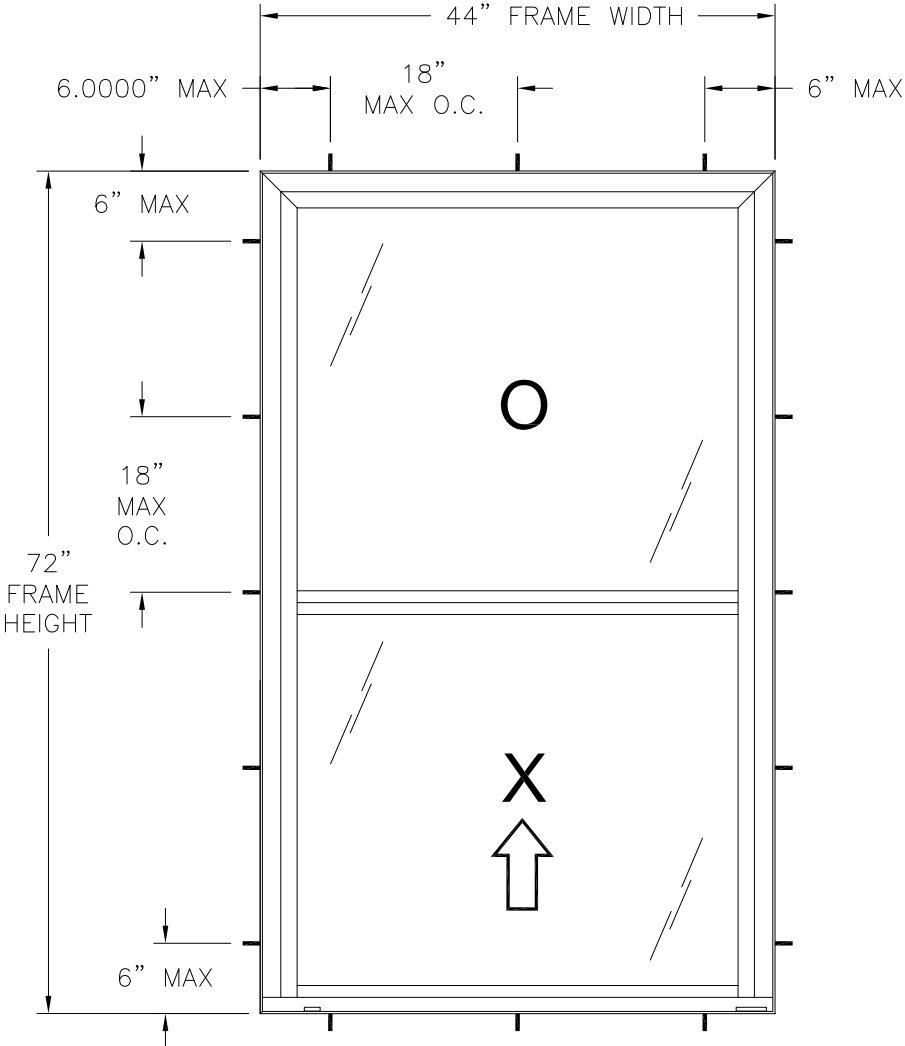
SERIES 450 SINGLE HUNG WINDOW EXTERIOR VIEW FRAME INSTALLATION
