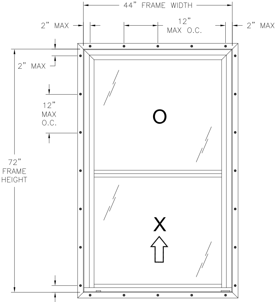
SERIES 450 SINGLE HUNG WINDOW EXTERIOR VIEW FIN INSTALLATION
