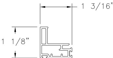
SASH STILE (V-705) EXTRUDED RIGID PVC
