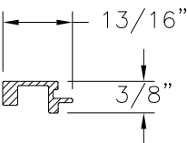
REINFORCEMENT (S-047) ALUMINUM 6061-T6
