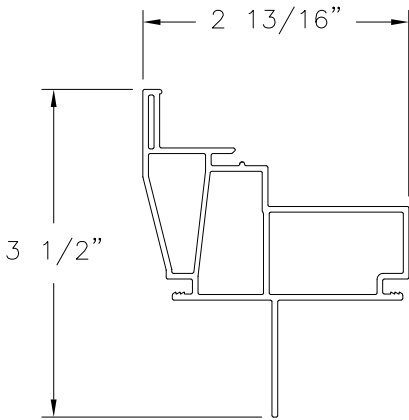
HEAD FRAME (V-770) FIN INSTALLATION EXTRUDED RIGID PVC
