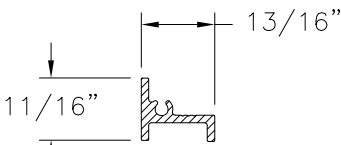
REINFORCEMENT (S-046) ALUMINUM 6061-T6
