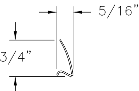
GLAZING BEAD (1718R) EXTRUDED RIGID PVC
