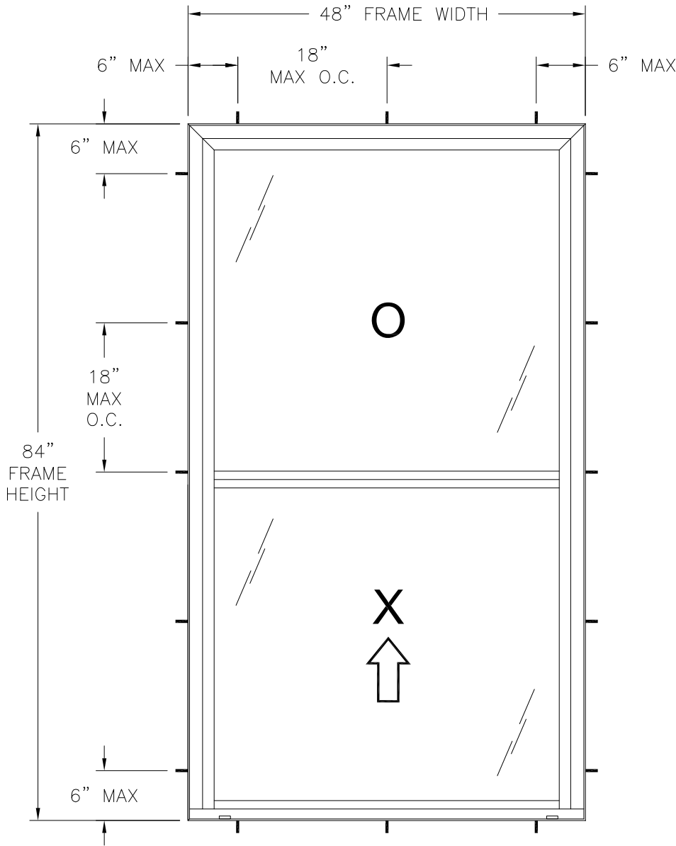
SERIES 450 SINGLE HUNG WINDOW EXTERIOR VIEW FRAME INSTALLATION
