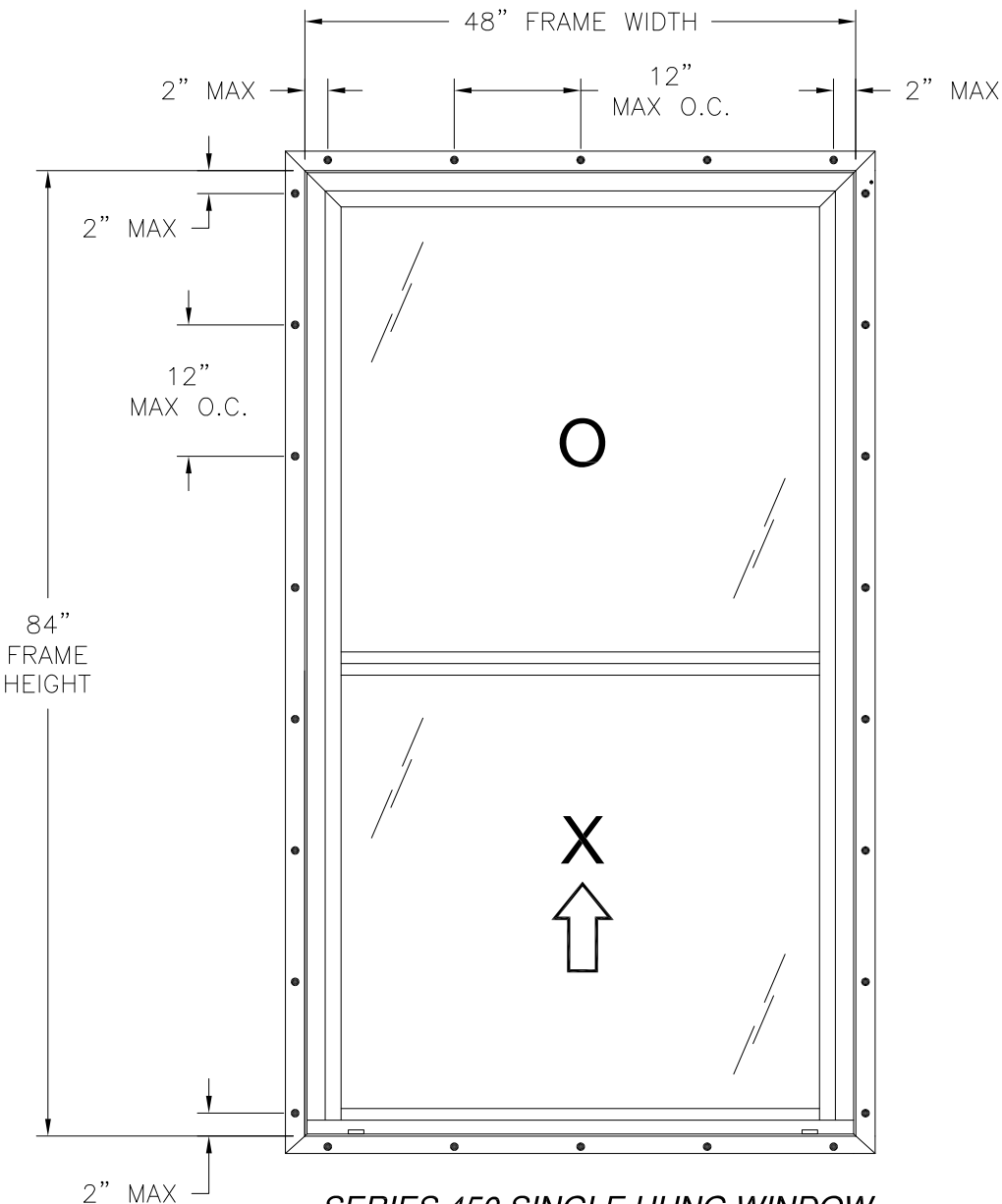
SERIES 450 SINGLE HUNG WINDOW EXTERIOR VIEW FIN INSTALLATION
