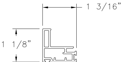
SASH STILE (V-705) EXTRUDED RIGID PVC
