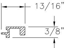
REINFORCEMENT (S-047) ALUMINUM 6061-T6
