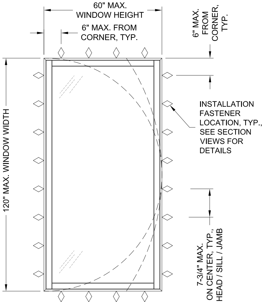
TYPICAL ELEVATION
