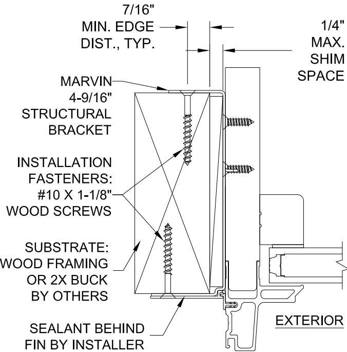
TYPICAL JAMB HORIZONTAL SECTION
