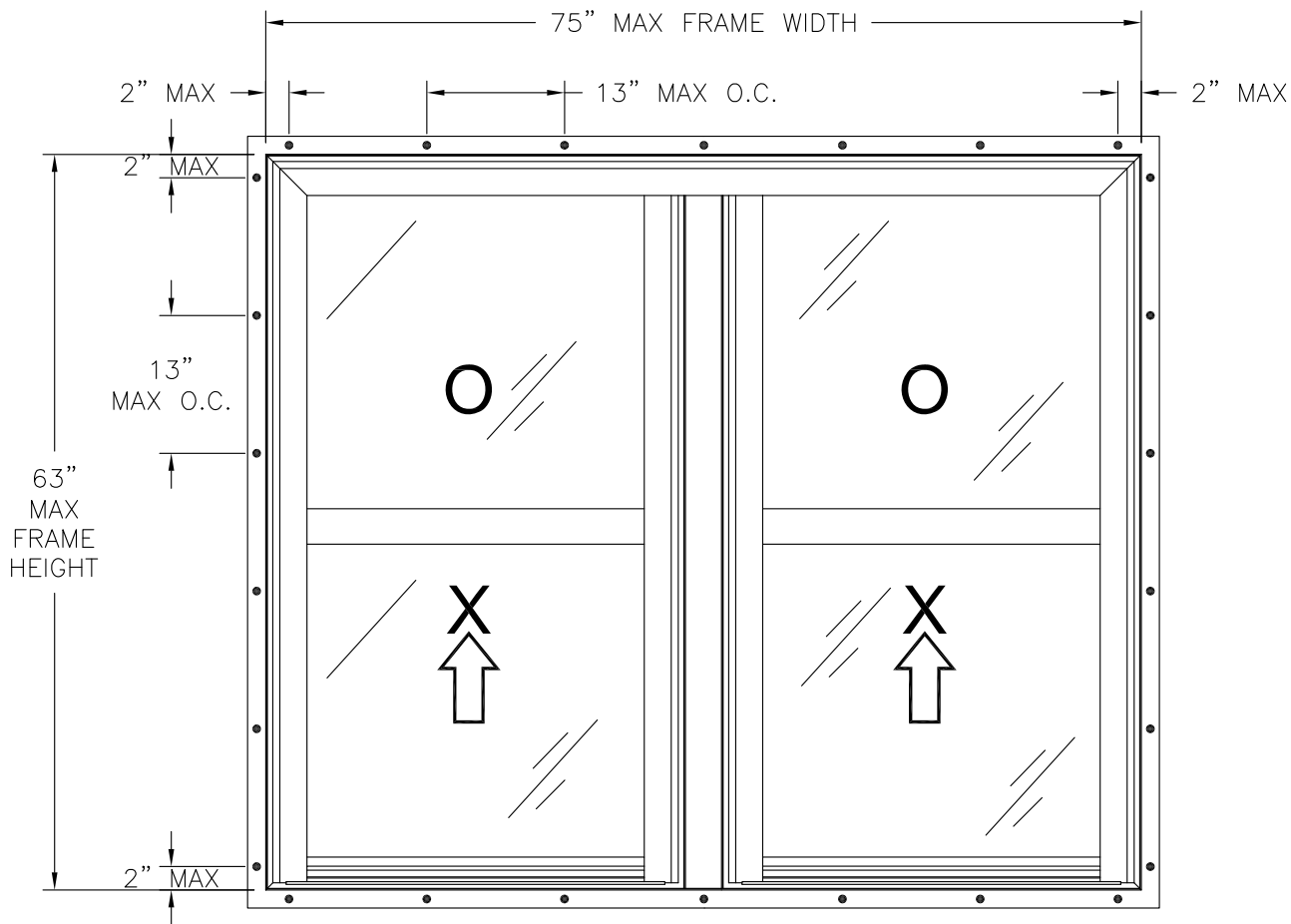
7122 UNIFRAME TWIN SINGLE HUNG EXTERIOR VIEW FIN INSTALLATION
