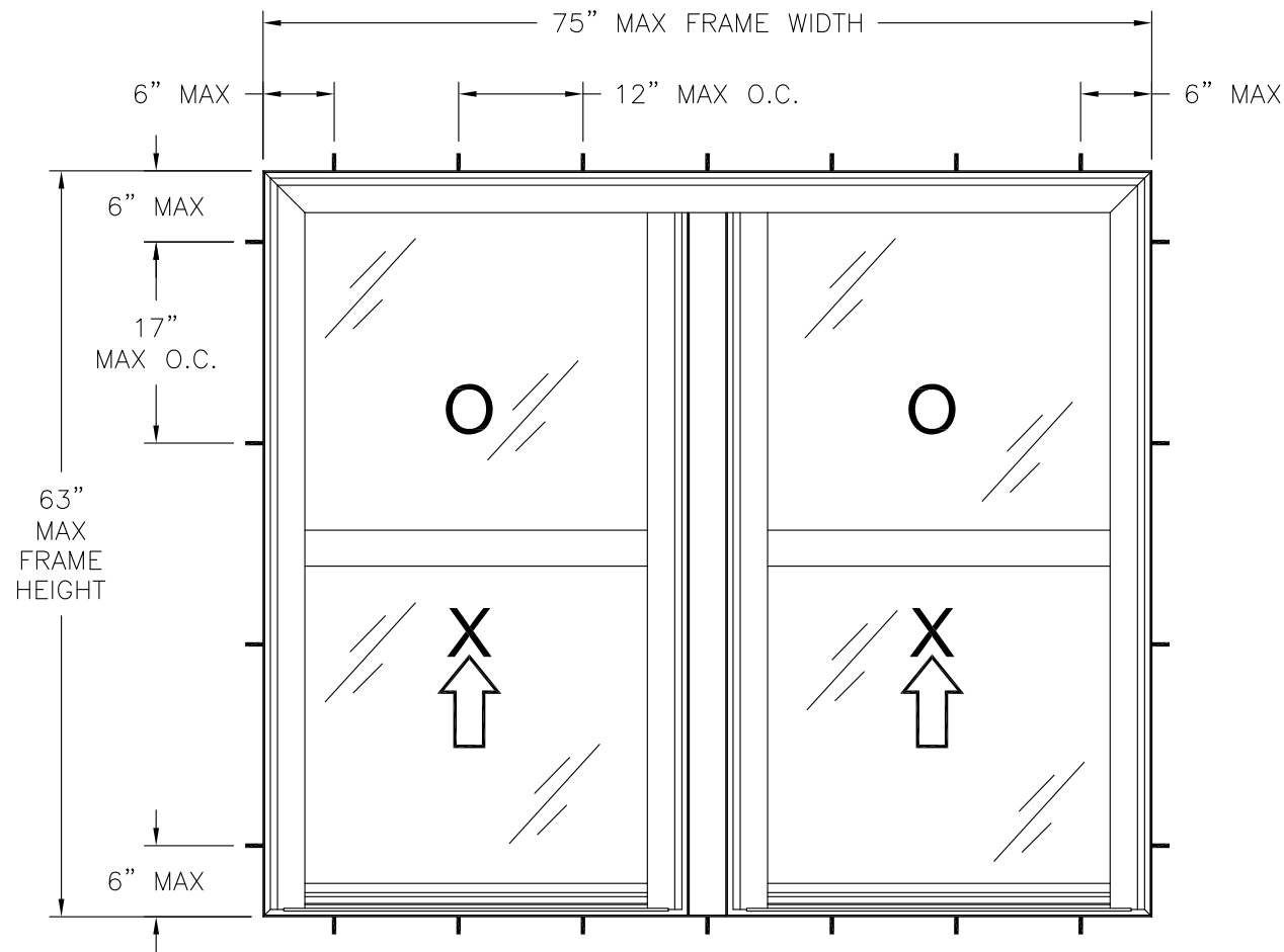
7122 UNIFRAME TWIN SINGLE HUNG EXTERIOR VIEW FRAME INSTALLATION
