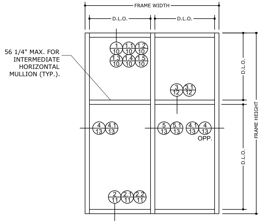
TYPICAL CURTAINWALL ELEVATION
