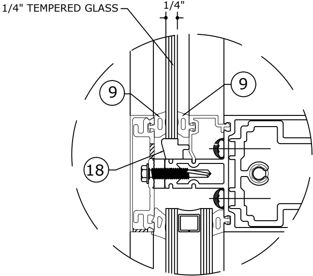
GLASS TYPE G2 GLAZING DETAIL N.T.S. GLASS RATING: NON IMPACT
