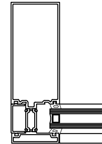
J1 DETAIL 4
