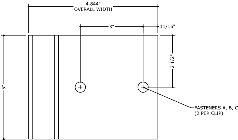
F ANCHOR CLIP DETAIL
