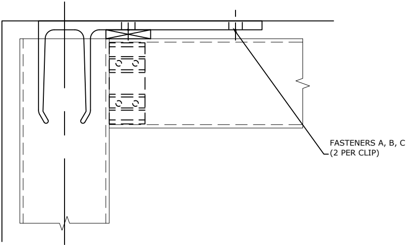
HEAD DETAIL
