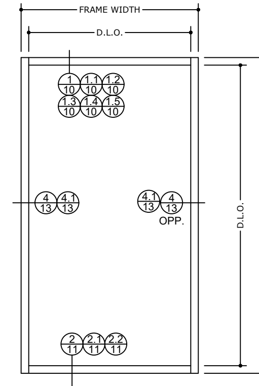
TYPICAL SINGLE PANEL ELEVATION
