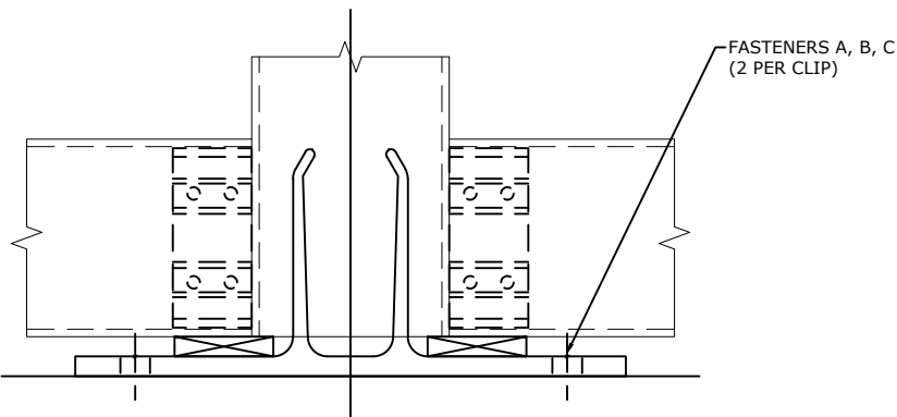
SILL DETAIL
