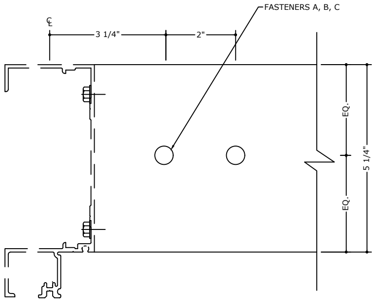
JAMB MULLION ANCHOR AT HEAD DETAIL
