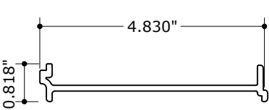
28 WW-251-01 SPLICE FOR WW-541
