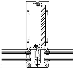
M1 CONTINUOUS OR SPLICED MULLION DETAILS 4.1, 4.4
