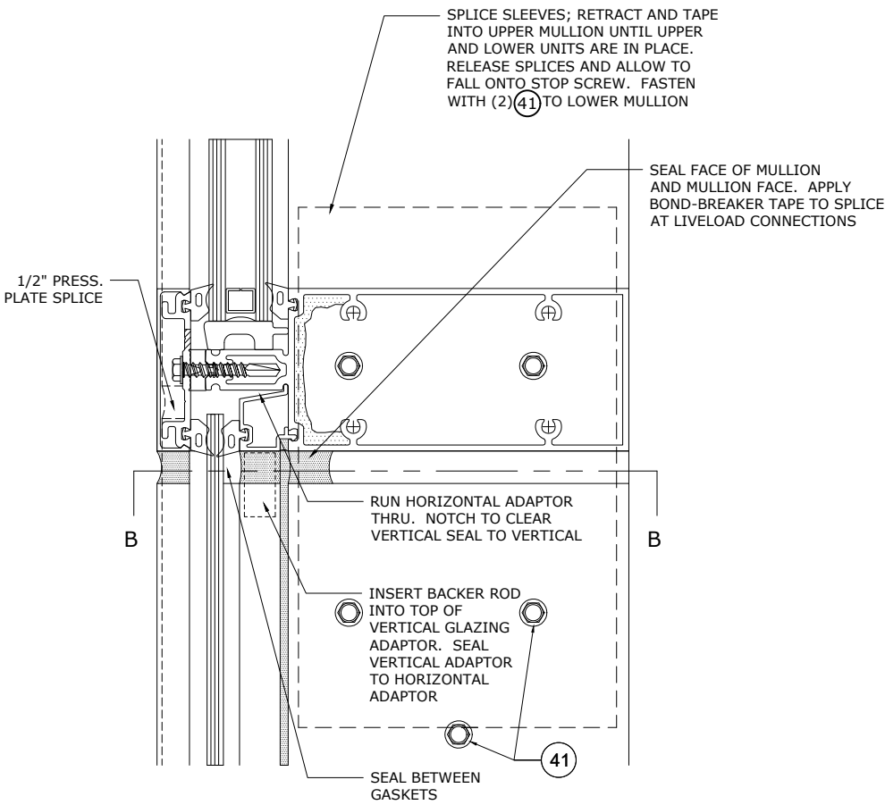
HARD SPLICE @ CAPTURED MULLION (JAMB SIM.)
