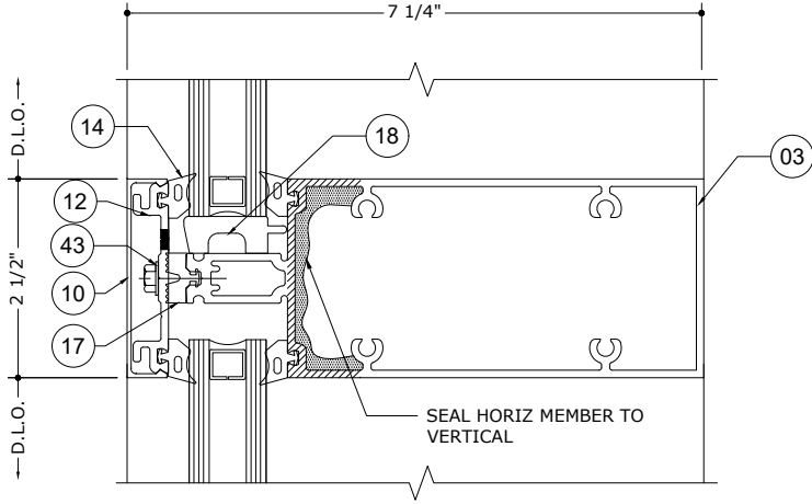
3.2 INTERMEDIATE HORIZONTAL DETAIL SCALE: 6" = 1'-0"
