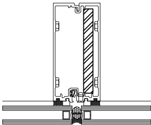
M2 SPLICED MULLION DETAIL 4.2, 4.5
