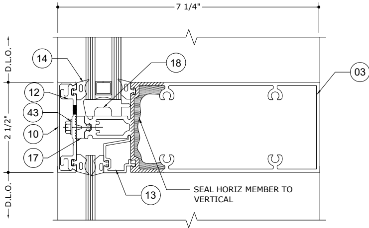
3 INTERMEDIATE HORIZONTAL DETAIL SCALE: 6" = 1'-0"
