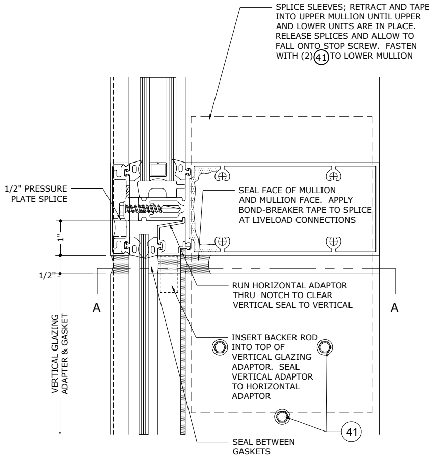
EXPANSION SPLICE @ CAPTURED MULLION
