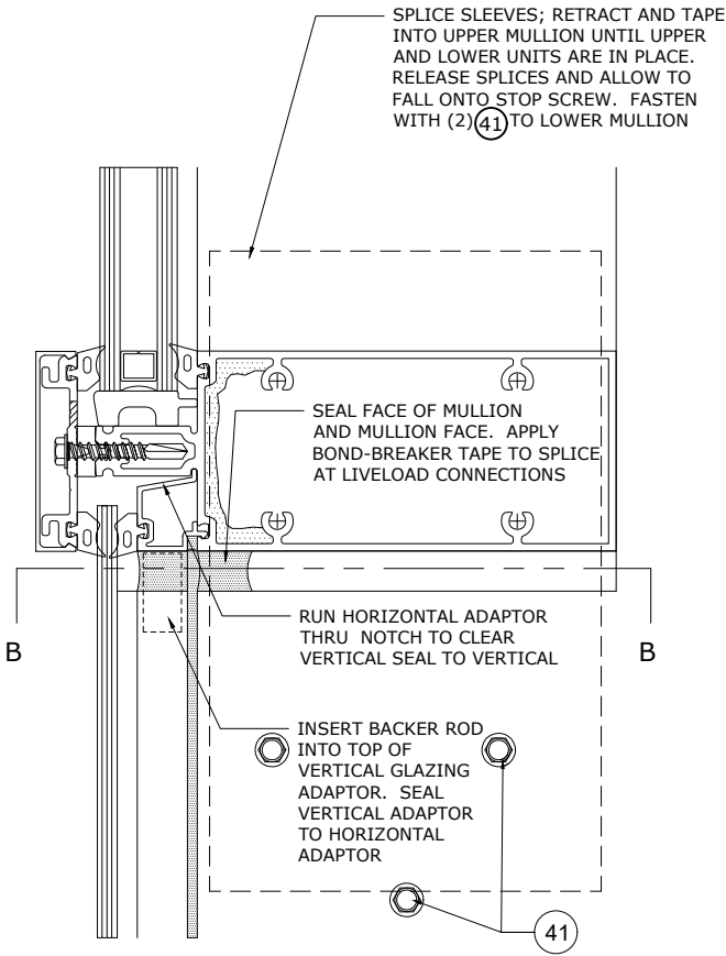
EXPANSION SPLICE @ SSG MULLION
