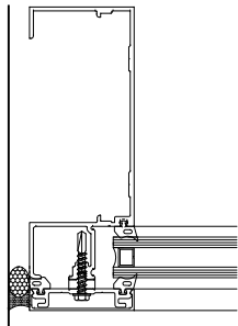
J1 CONTINUOUS OR SPLICED JAMB DETAILS 4, 4.3
