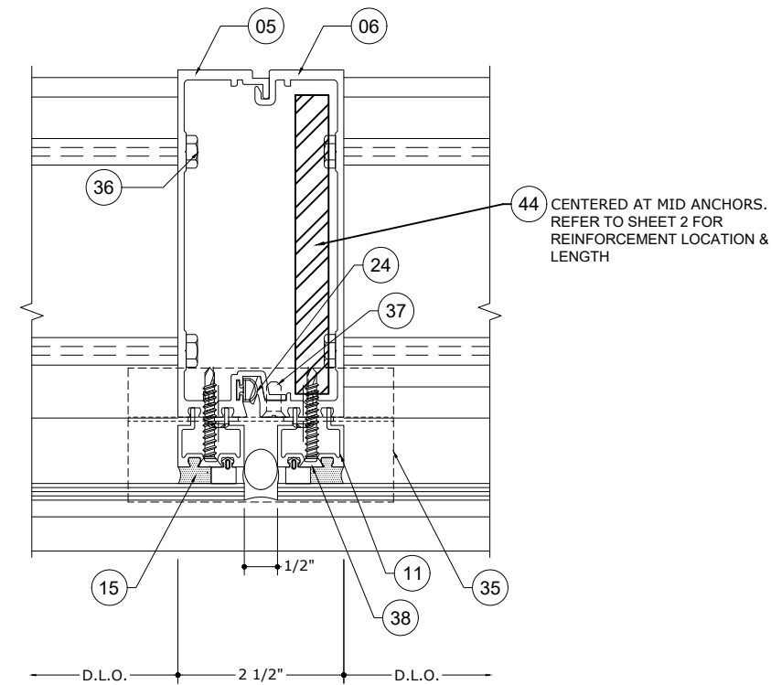
4.9 SSG VERTICAL DETAIL - M2
