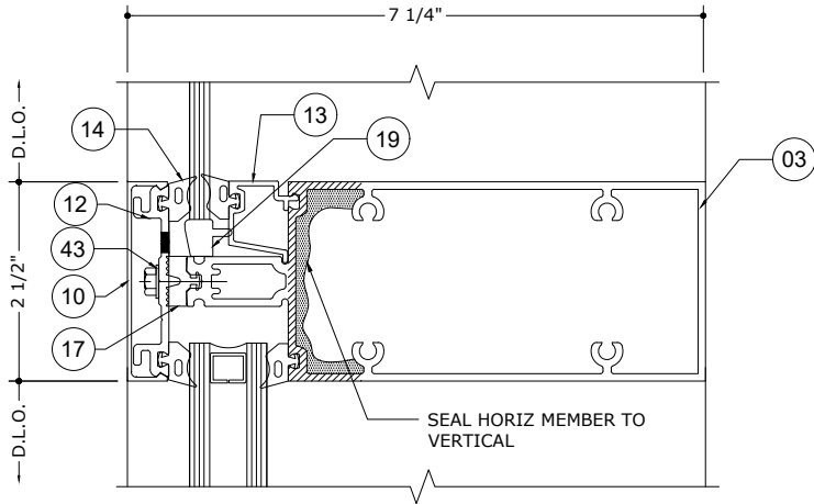
3.1 INTERMEDIATE HORIZONTAL DETAIL SCALE: 6" = 1'-0"
