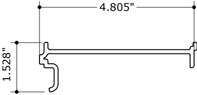
27 WW-250-01 SPLICE FOR WW-540
