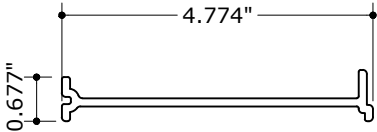
31 WW-255-01 SPLICE FOR WW-545
