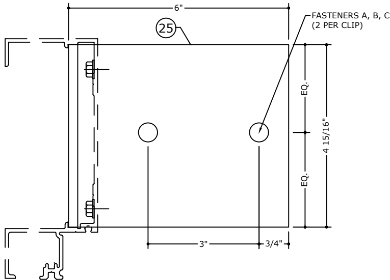
JAMB MULLION ANCHOR AT HEAD DETAIL
