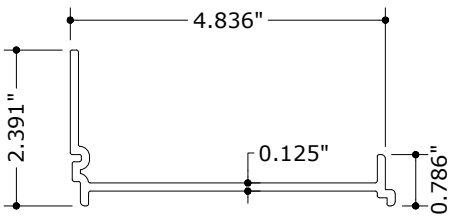
29 WW-253-01 SPLICE FOR WW-543
