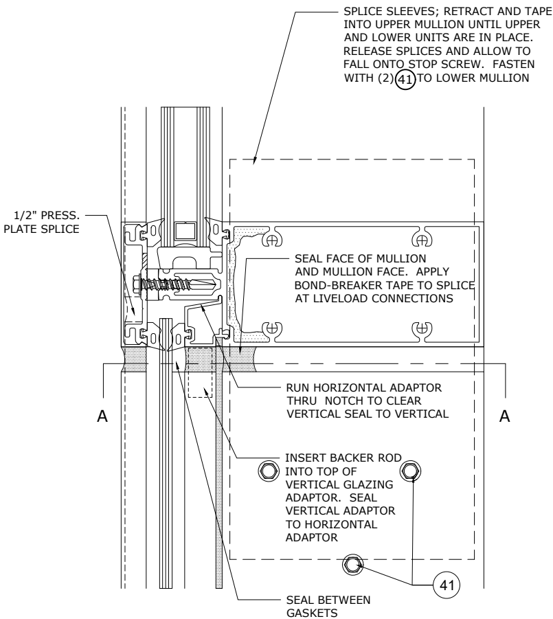
EXPANSION SPLICE @ JAMB MULLION
