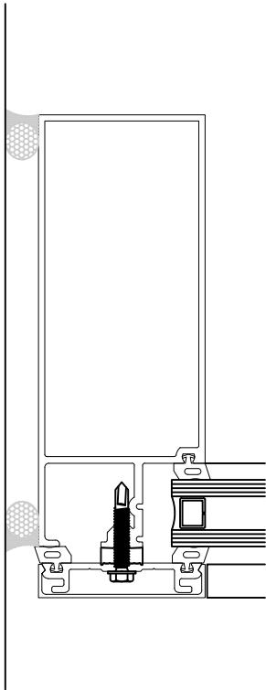
J1 CONTINUOUS OR SPliced JAMB
