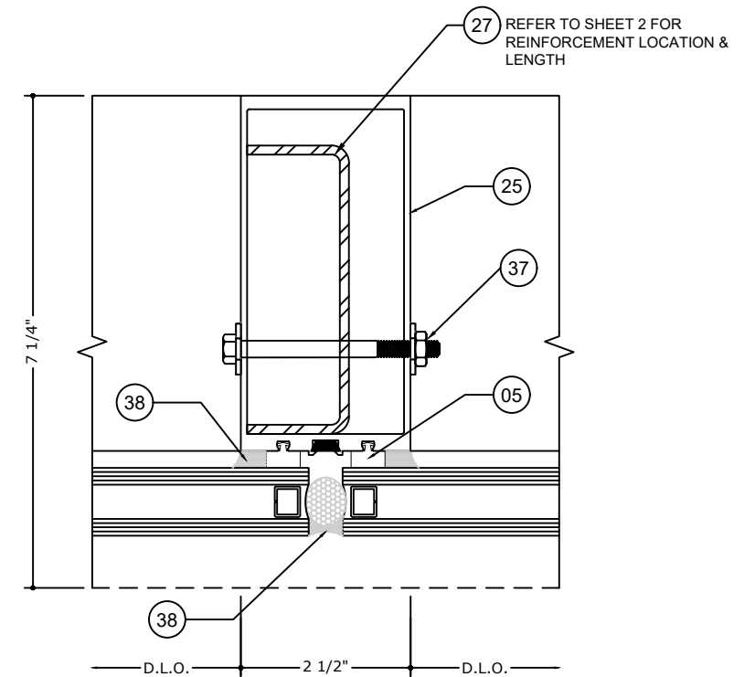
5.2 INTERMEDIATE VERTICAL DETAIL - M2
