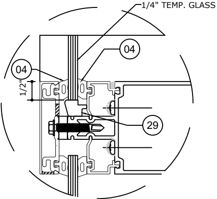
GLASS TYPE G2 GLAZING DETAIL N.T.S. GLASS RATING: NON-IMPACT
