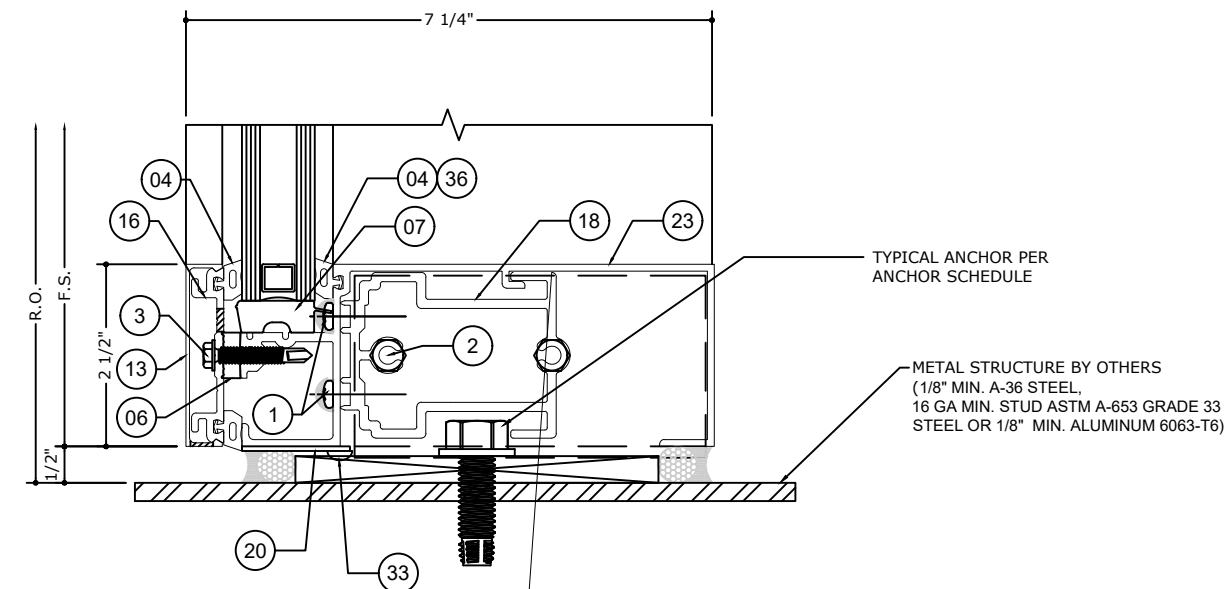
2.2 SILL DETAIL
