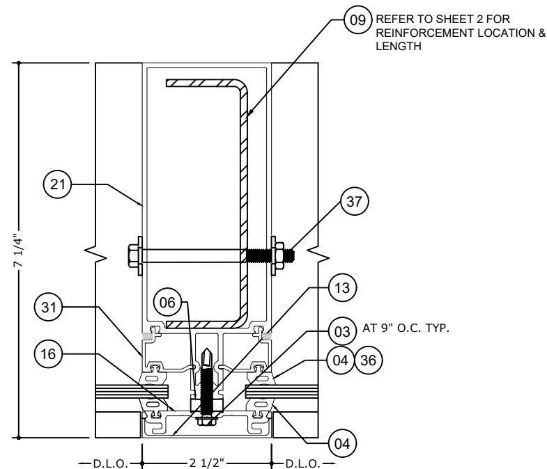
5.3 INTERMEDIATE VERTICAL DETAIL - M1
