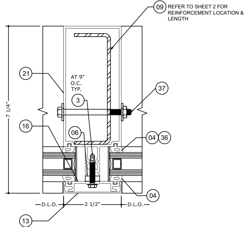
5.1 INTERMEDIATE VERTICAL DETAIL - M1
