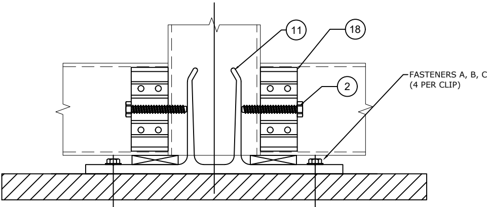
INTERMEDIATE MULLION SILL DETAIL
