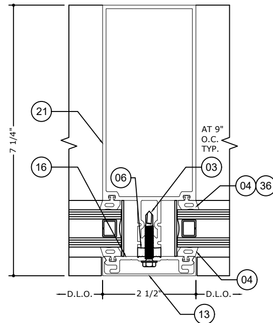
5 INTERMEDIATE VERTICAL DETAIL
