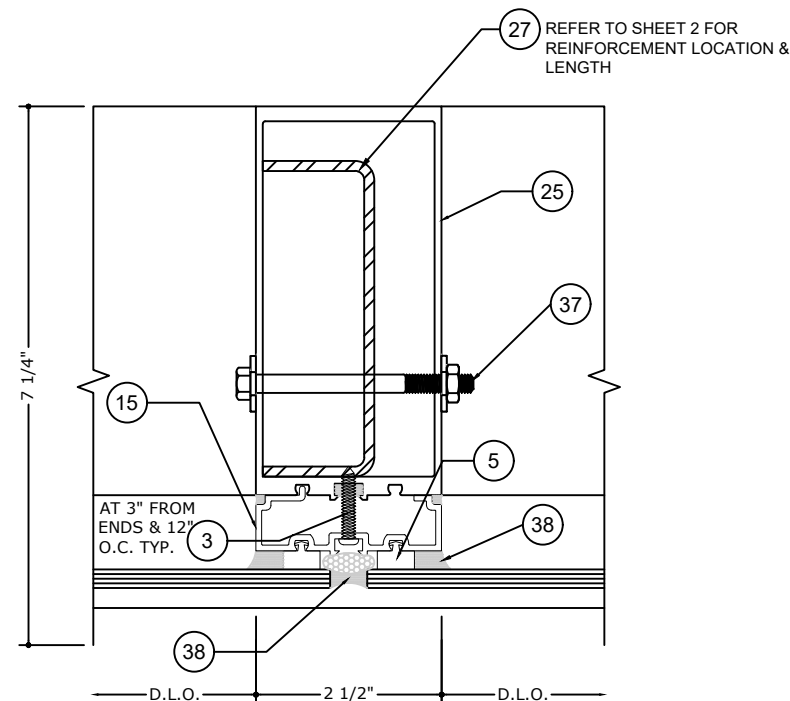
5.4 INTERMEDIATE VERTICAL DETAIL - M2
