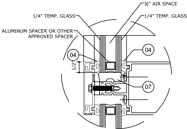
GLASS TYPE G1 GLAZING DETAIL N.T.S. GLASS RATING: NON-IMPACT
