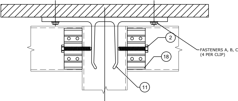
INTERMEDIATE MULLION HEAD DETAIL
