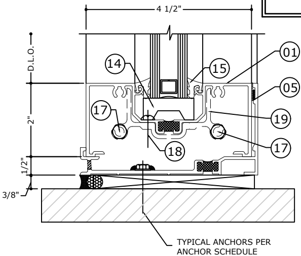
2.2 SILL DETAIL
