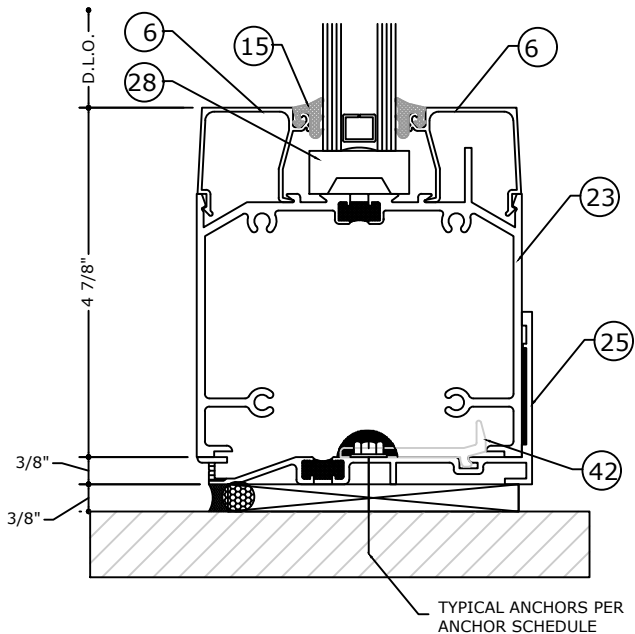
2.5 SILL DETAIL LIMITED TO +25 / -25 P.S.F
