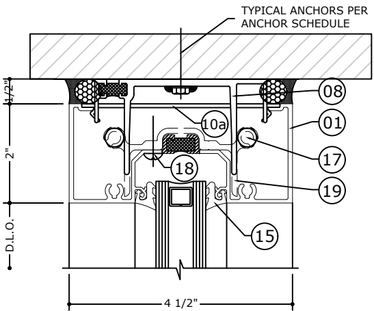
1 HEAD DETAIL
