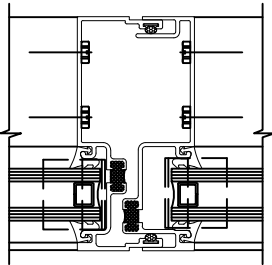
M4 FRONT & BACK DETAILS 8.2, 12.2 (FRONT SET SHOWN)
