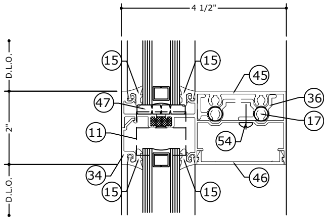
7 HORIZONTAL DETAIL
