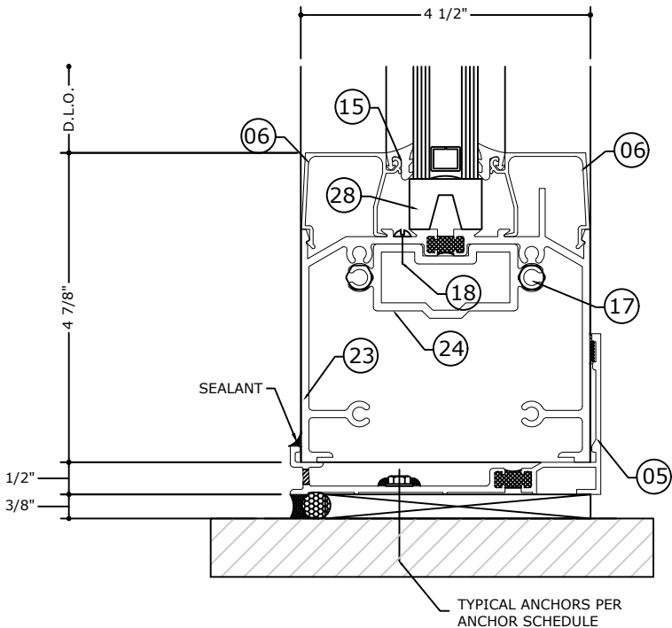
2.4 SILL DETAIL
