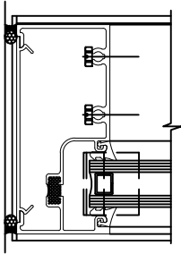
J2 DETAILS 8, 12 (FRONT SET SHOWN)
