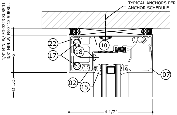
1.1 HEAD DETAIL
