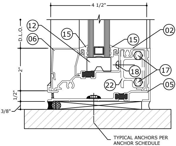
2 SILL DETAIL
