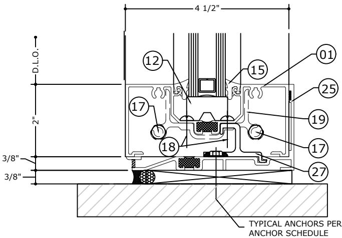
2.3 SILL DETAIL LIMITED TO +25 / -25 P.S.F
