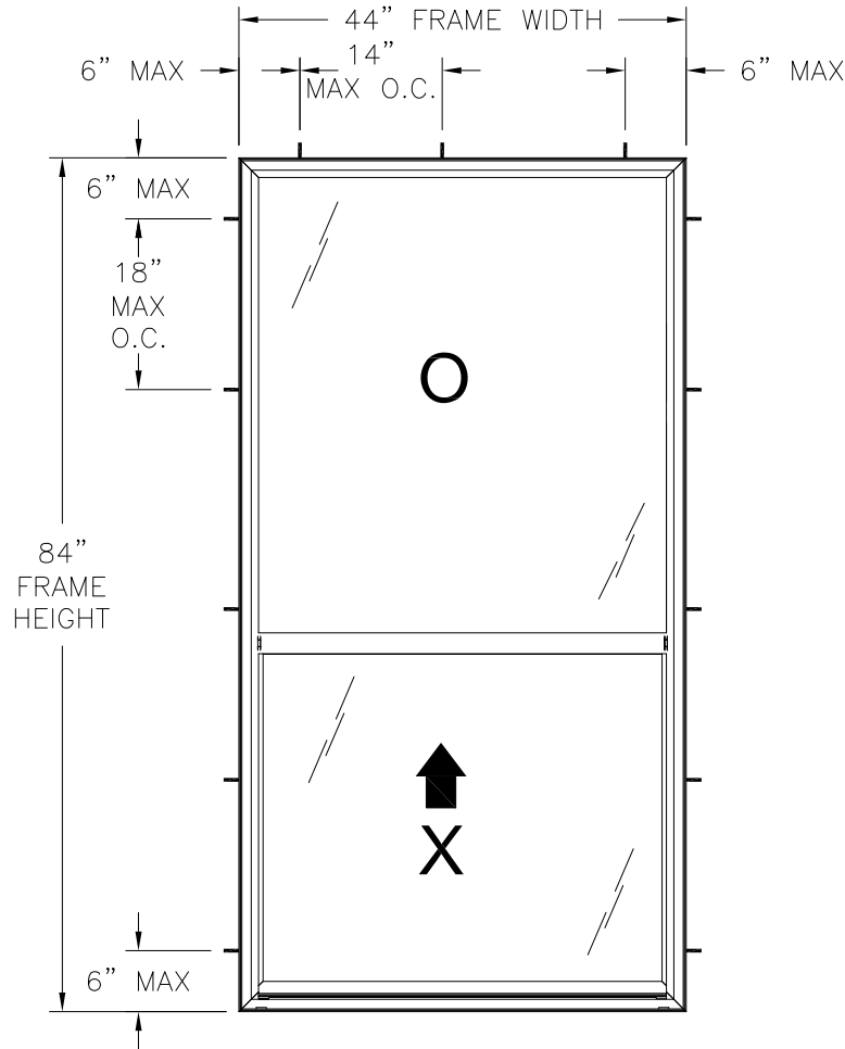
SERIES 3540 PVC SH WINDOW FRAME INSTALLATION EXTERIOR VIEW
