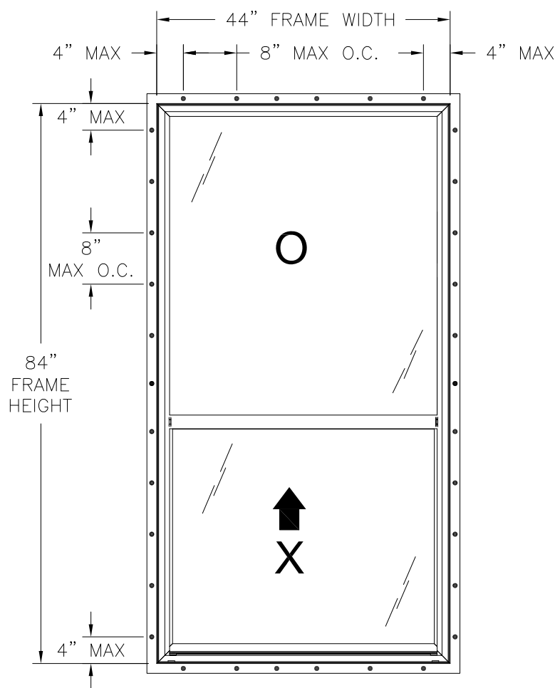
SERIES 3540 PVC SH WINDOW FIN INSTALLATION EXTERIOR VIEW
