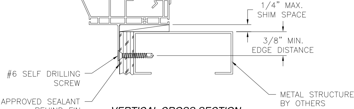
VERTICAL CROSS SECTION METAL STRUCTURE INSTALLATION
