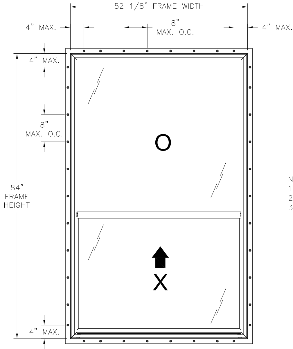
SERIES 3540 PVC SINGLE HUNG WINDOW EXTERIOR VIEW
