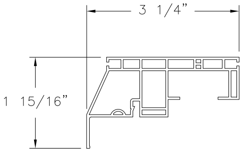
MAIN FRAME PVC (V-634)
