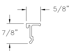
LIFT BEAD PVC (V-817)
