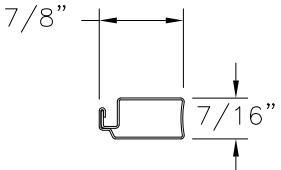
MEETING RAIL LINER STEEL .019" THICK (RF-104S)
