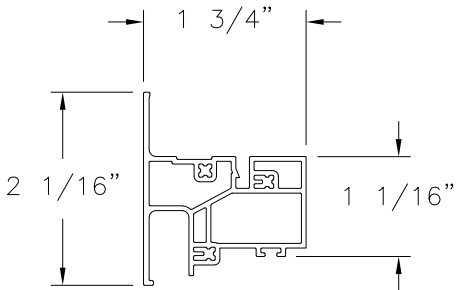
FIXED MEETING RAIL PVC (V-321)
