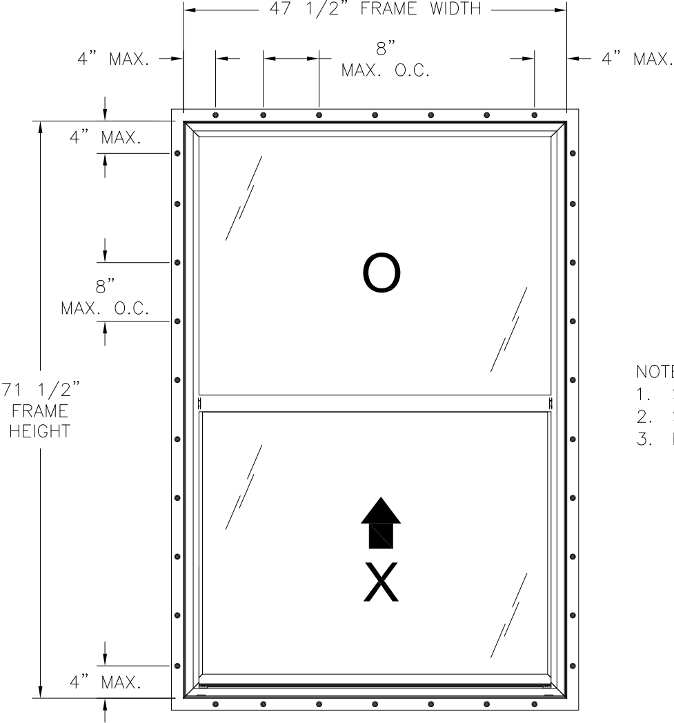
SERIES 3540 PVC SINGLE HUNG WINDOW EXTERIOR VIEW
