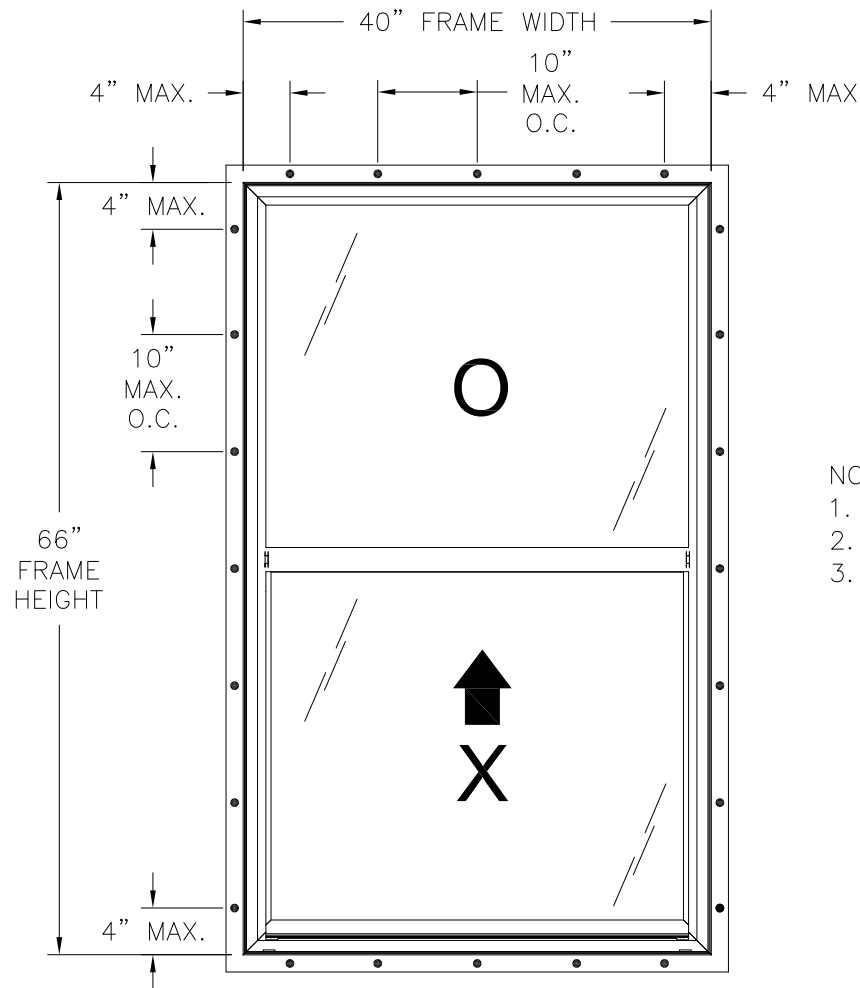
SERIES 3540 PVC SINGLE HUNG WINDOW EXTERIOR VIEW
