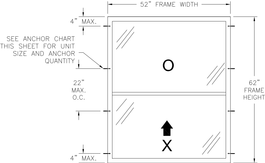
SERIES 3540 FINLESS PVC SINGLE HUNG WINDOW EXTERIOR VIEW
