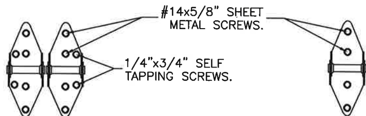
14 GA. DOUBLE END HINGES VIEW "A"
