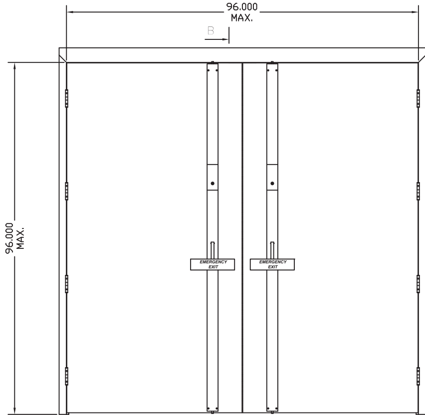
OUTSWING DOORS WITH VERTICALLY MOUNTED DEVICES
