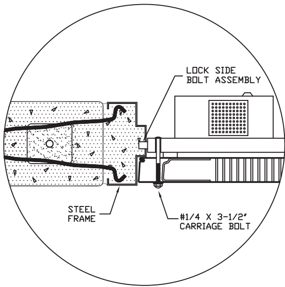
SECTION A-A HORIZONTAL DEVICE POSITIVE LOCK THPA(H)-40 LOCK SIDE
