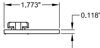
4 CLADDING FASTENER E41-0116 PLASTIC GF 30
