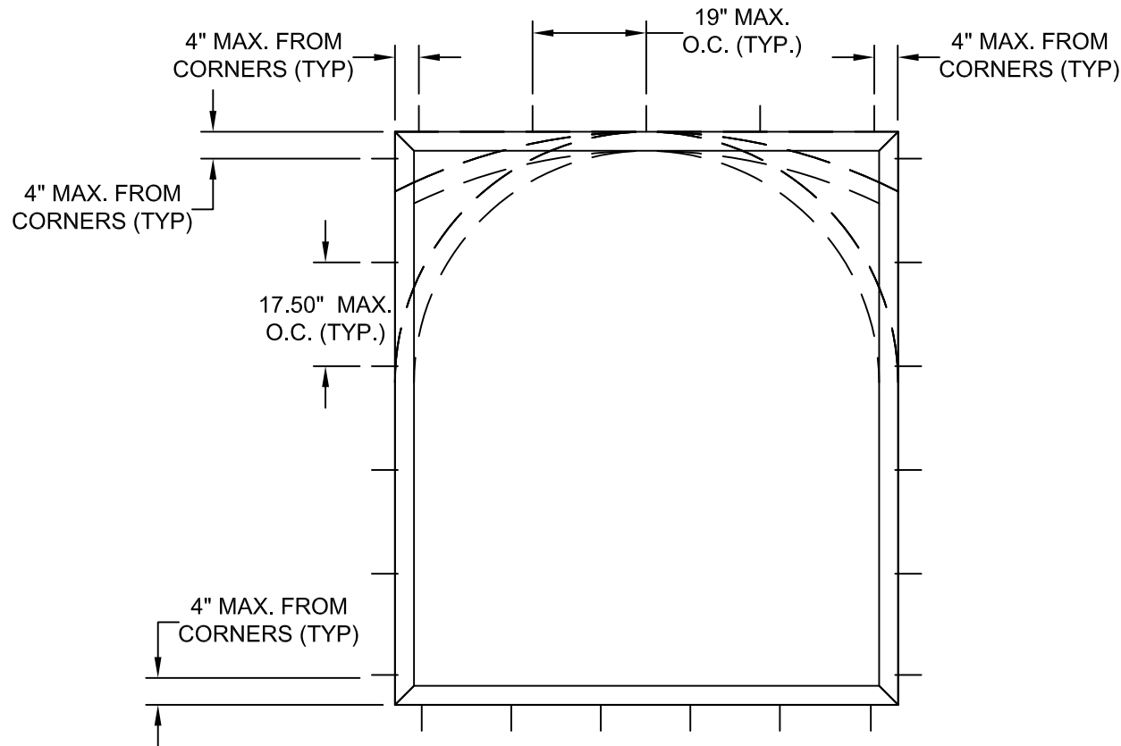
CLIP INSTALLATION ANCHOR ELEVATION EXTERIOR VIEW
