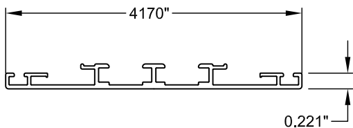
13 MUNTIN CLADDING PROFILE E51-0004 ALUMINUM 6060 T5 0.055" THICK
