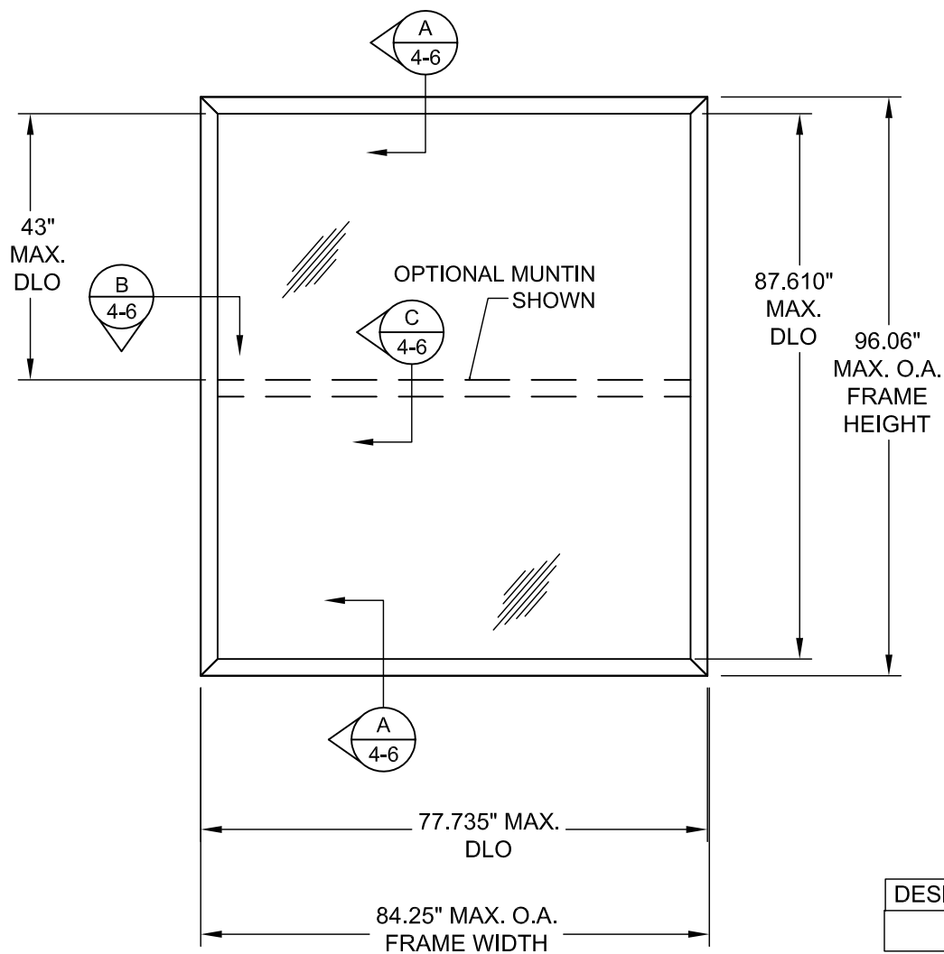
SERIES "F" ALUMINUM CLAD WOOD FIXED WINDOW WINDOW ELEVATION EXTERIOR VIEW
