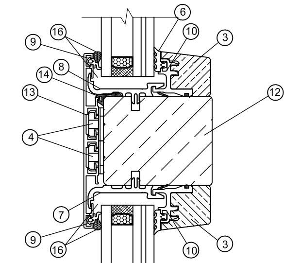
MUNTIN CROSS SECTION
