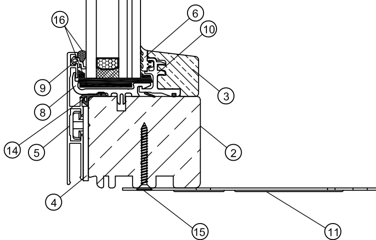
VERTICAL CROSS SECTION
