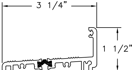
SILL S56829 & 56828 ALUMINUM 6063-T6 .125" THICK
