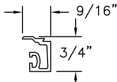
GLASS STOP S34713 ALUMINUM 6063-T6 .060" THICK
