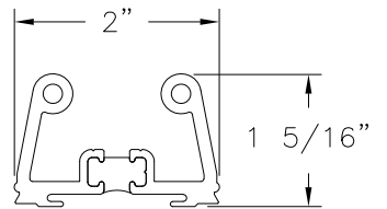
FRAME LUG H10268 ALUMINUM 6063-T6 .125" THICK
