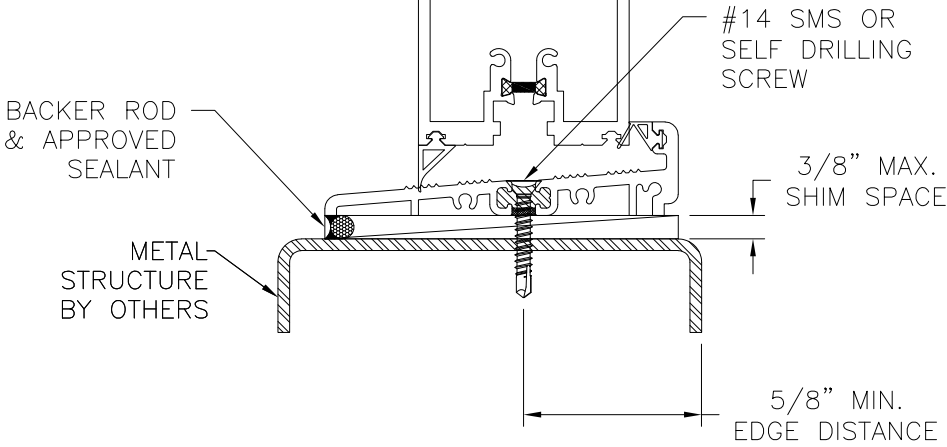
VERTICAL CROSS SECTION METAL STRUCTURE INSTALLATION FOR SILL DETAIL WITH 1.5" HIGH PERFORMANCE, SEE SHEET 8
