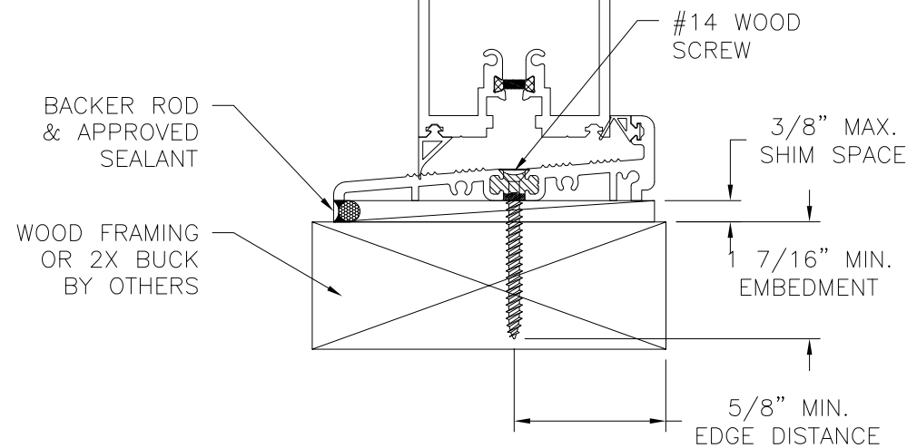
VERTICAL CROSS SECTION WOOD FRAMING OR 2X BUCK INSTALLATION FOR SILL DETAIL WITH 1.5" HIGH PERFORMANCE, SEE SHEET 8
