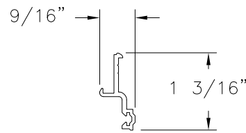
CHASE S46534 ALUMINUM 6063-T6 .070" THICK
