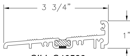
SILL S46538 ALUMINUM 6063-T6 .125" THICK
