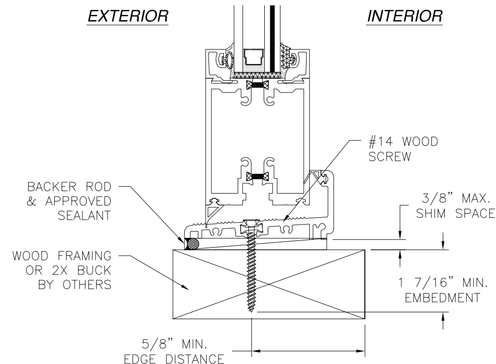
VERTICAL CROSS SECTION WOOD FRAMING OR 2X BUCK INSTALLATION WITH 1.5" HIGH PERFORMANCE
