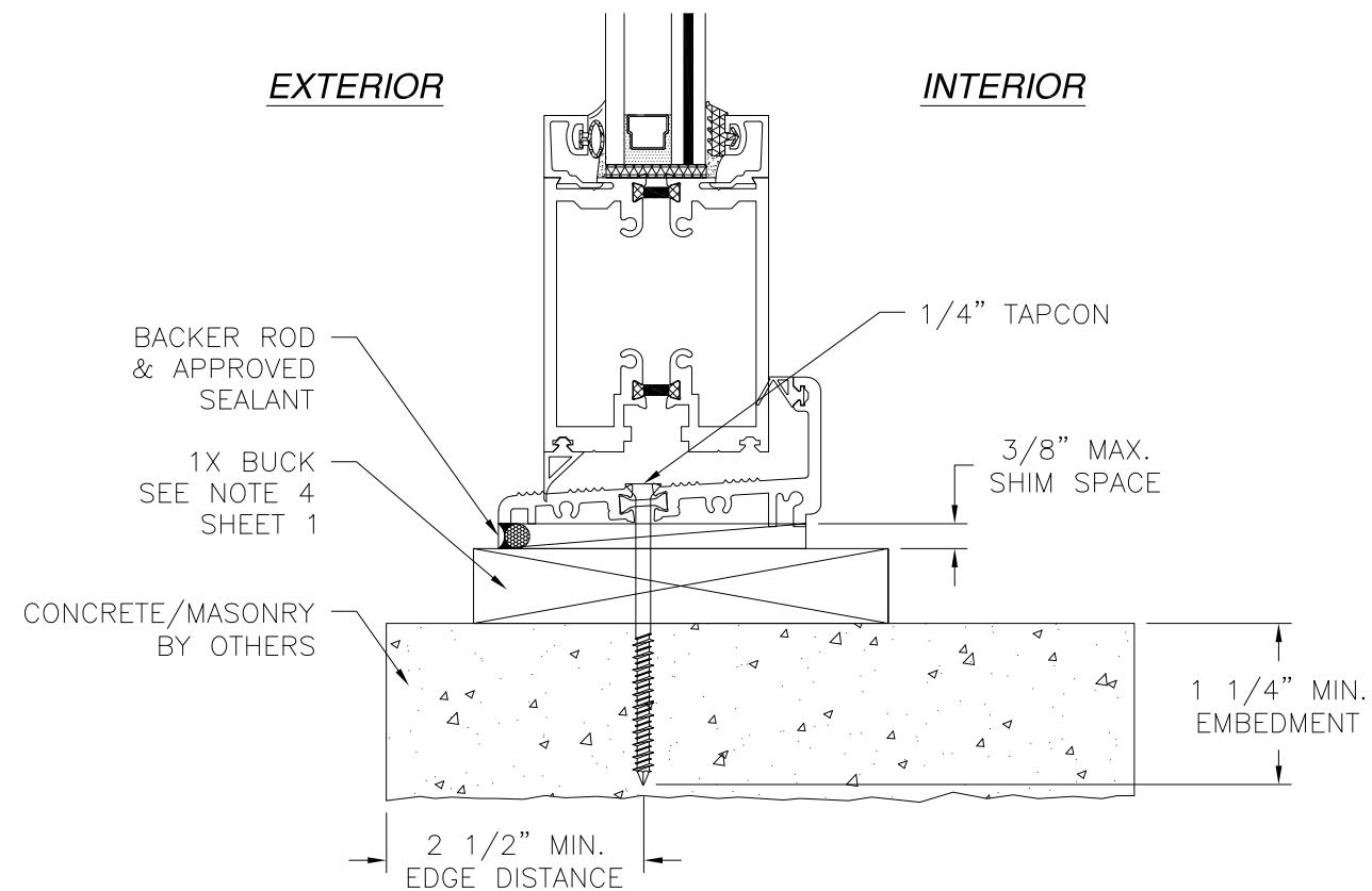
VERTICAL CROSS SECTION CONCRETE/MASONRY WITH 1X BUCK INSTALLATION WITH 1.5" HIGH PERFORMANCE
