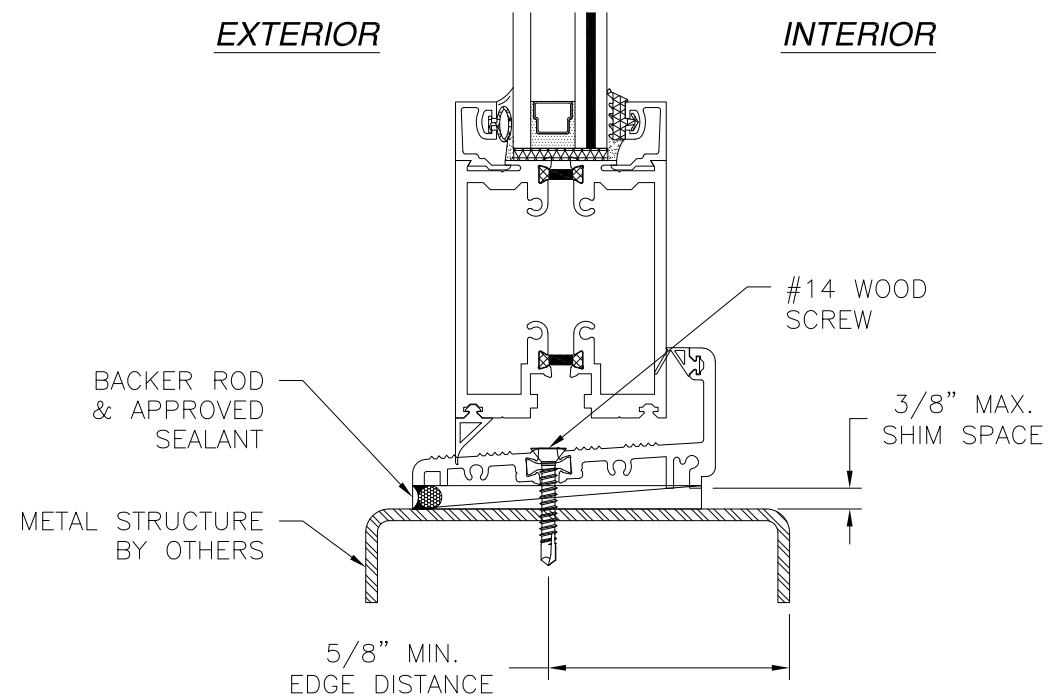
VERTICAL CROSS SECTION METAL STRUCTURE INSTALLATION WITH 1.5" HIGH PERFORMANCE
