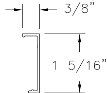
CAP 51741 ALUMINUM 6063-T6 .050" THICK
