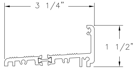
G3 HP OUT-SWING SILL 56829 & 56828 ALUMINUM 6063-T6 .125" THICK
