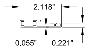
39 E51-0074 MEETING STILE CLAD ALUMINUM 6060-T66
