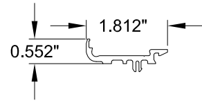
25 E51-0189 BASE FASTENER FOR GLASS BOTTOM
