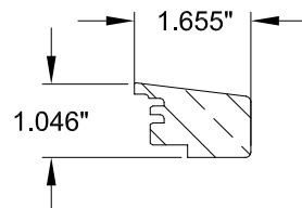
18 F33-0111 32MM GLAZING BEAD WOOD G.50
