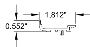
24 E51-0185 BASE FASTENER FOR GLASS FIXED SIDE/TOP
