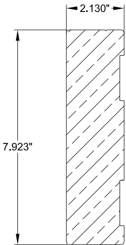
1 F33-0001 FRAME LOCK JAMB WOOD G.50
