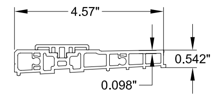
45 E33-4002 ATTACHMENT BAR ALUMINUM 6060-T66
