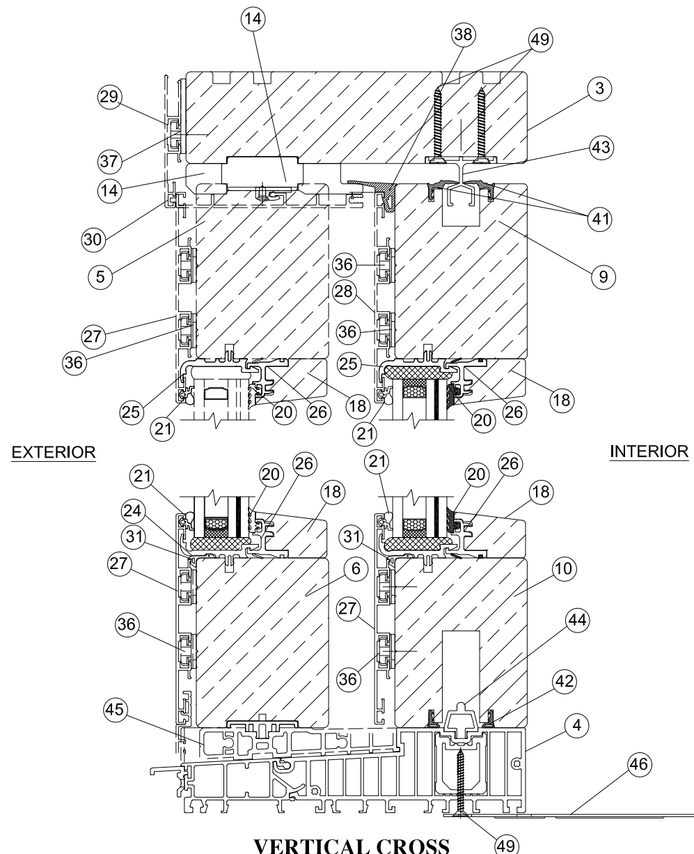
VERTICAL CROSS SECTION FOR PARTS IDENTIFICATION
