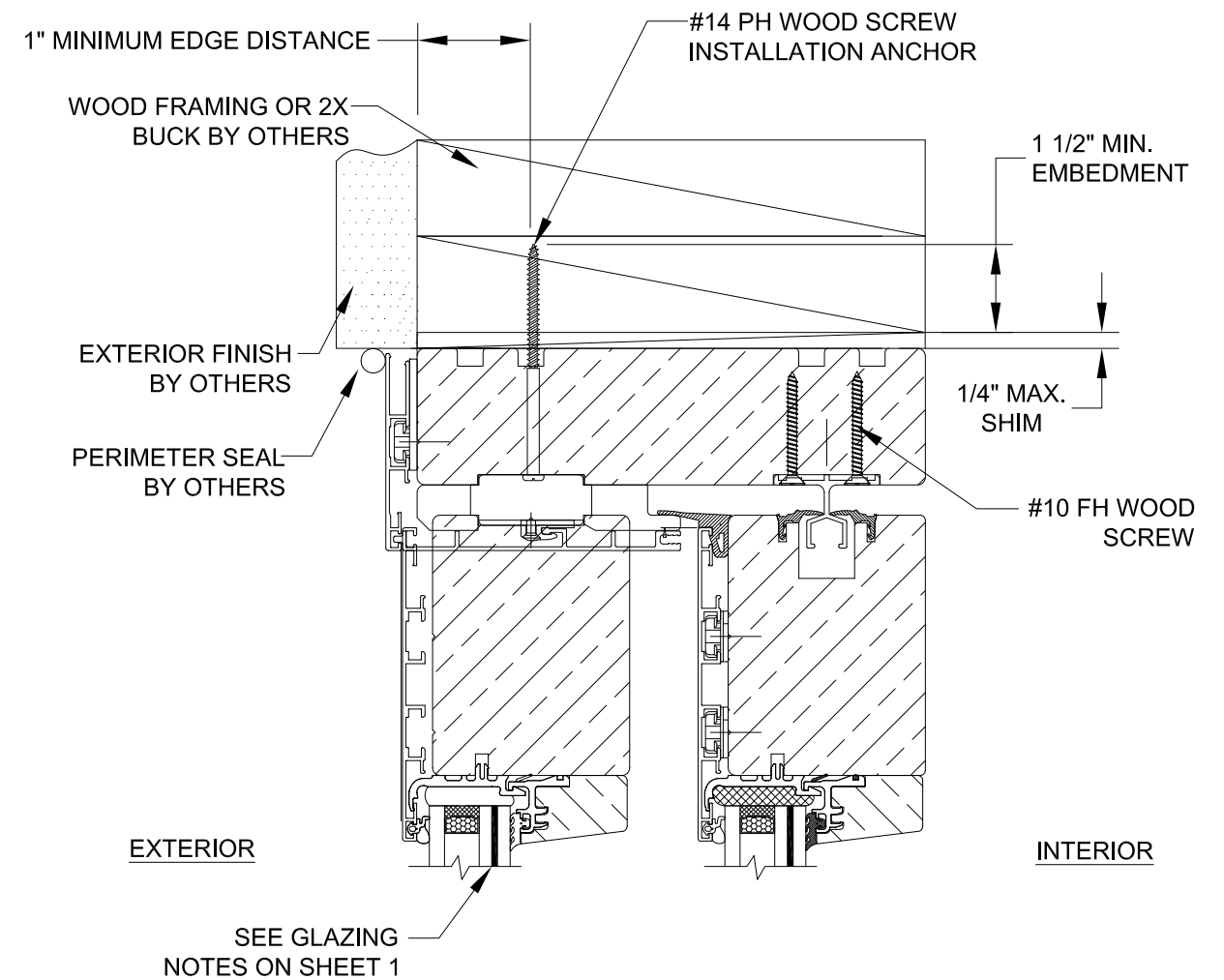
B 4 VERTICAL SECTION 2X WOOD SUBSTRATE FRAME INSTALLATION
