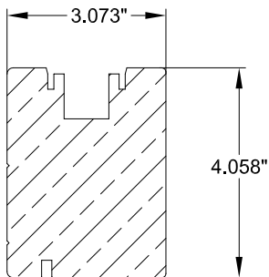
9 F33-0308 OPERABLE SASH TOP RAIL WOOD G.50
