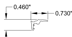
41 E33-1004 TOP GUIDE RAIL GASKET EPDM 70 DUR.
