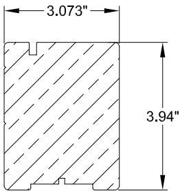
6 F33-0005 FXD. SASH BOTTOM WOOD G.50
