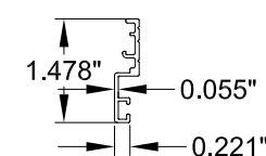
33 E33-0004-1 BOTTOM PROFILE FIXED ALUMINUM 6060-T66
