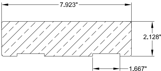
3 F33-0003 FRAME HEAD WOOD G.50
