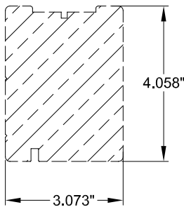
5 F33-0304 FIXED SASH TOP WOOD G.50
