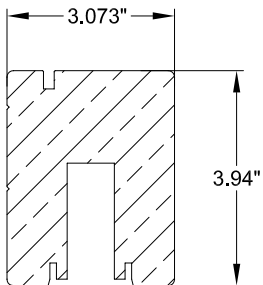
10 F33-0009 OPERABLE SASH BOTTOM RAIL WOOD G.50
