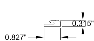
19 E41-0151 HOLDER FOR ENLARGEMENT PROFILE
