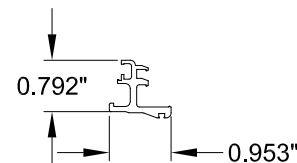
26 E51-0187 BASE FASTENER FOR BASE
