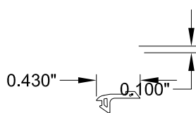
31 E41-1028 SASH GLAZING GASKET EPDM 70 DUR.
