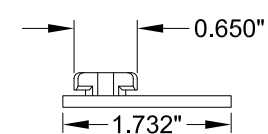
37 E41-0116 CLADDING FASTENER PLASTIC
