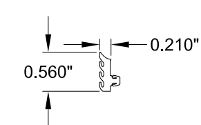
20 E41-1002 INTERIOR GLAZING GASKET EPDM 80 DUR.
