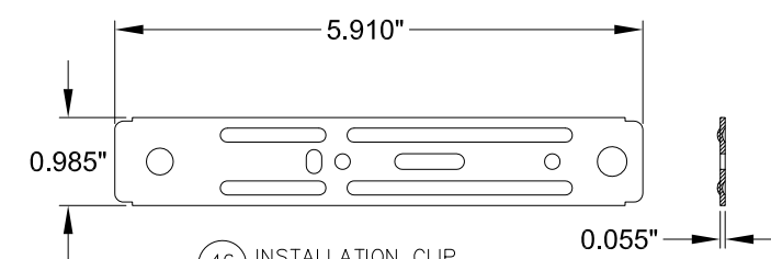
46 INSTALLATION CLIP GALVANIZED STEEL 0.0551\" THICK
