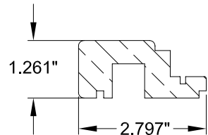
17 F33-0337 FILLER BEAD MIDDLE TRACK 1 WOOD G.50
