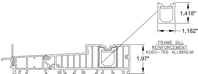
4 FRAME SILL SEGMENT 6060-T66 ALUMINUM E33-4001
