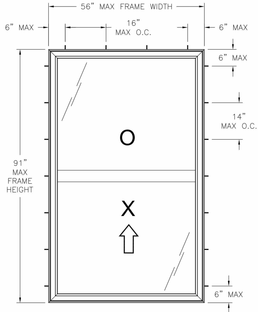
CAMBRIDGE SINGLE HUNG EXTERIOR VIEW FRAME INSTALLATION
