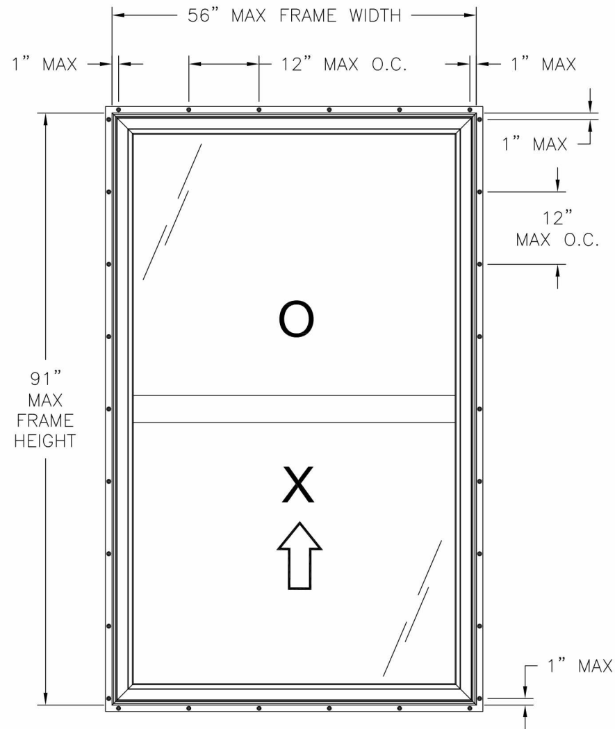
S-SERIES SINGLE HUNG EXTERIOR VIEW FIN INSTALLATION
