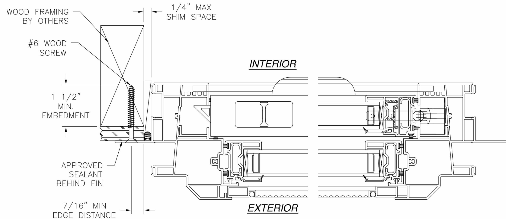
JAMB INSTALLATION DETAIL WOOD FRAMING OR 2X BUCK INSTALLATION
