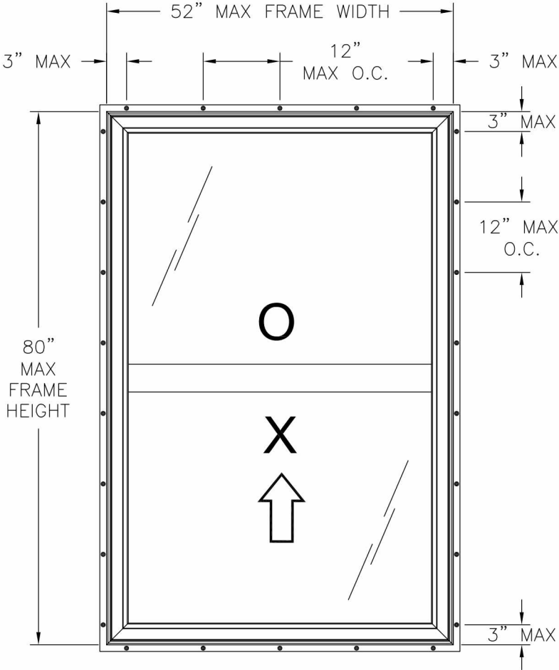
S-SERIES SINGLE HUNG EXTERIOR VIEW FIN INSTALLATION
