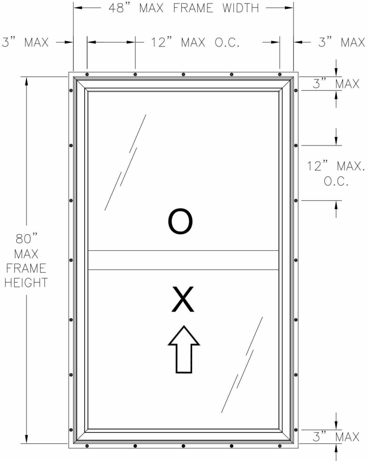
S-SERIES SINGLE HUNG EXTERIOR VIEW FIN INSTALLATION
