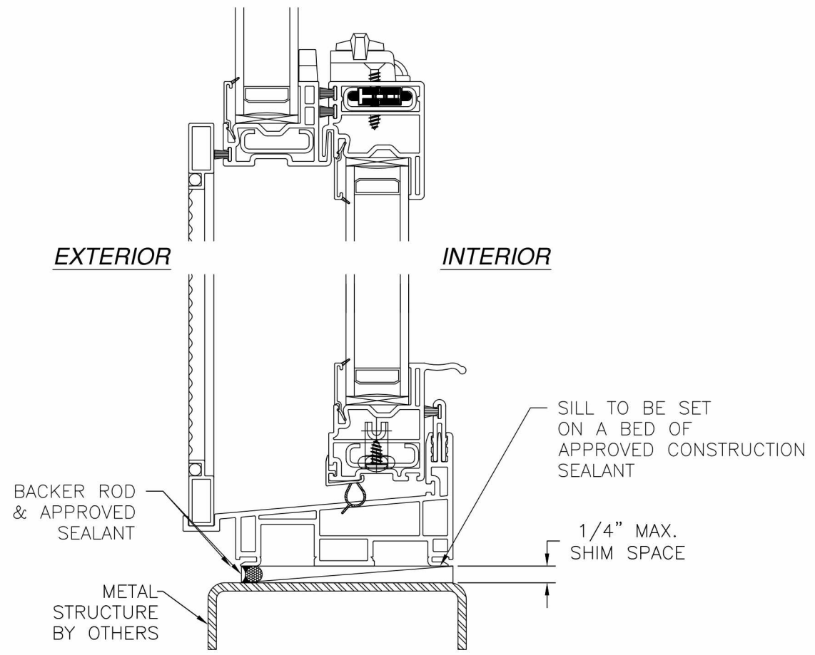
VERTICAL CROSS SECTION METAL STRUCTURE INSTALLATION
