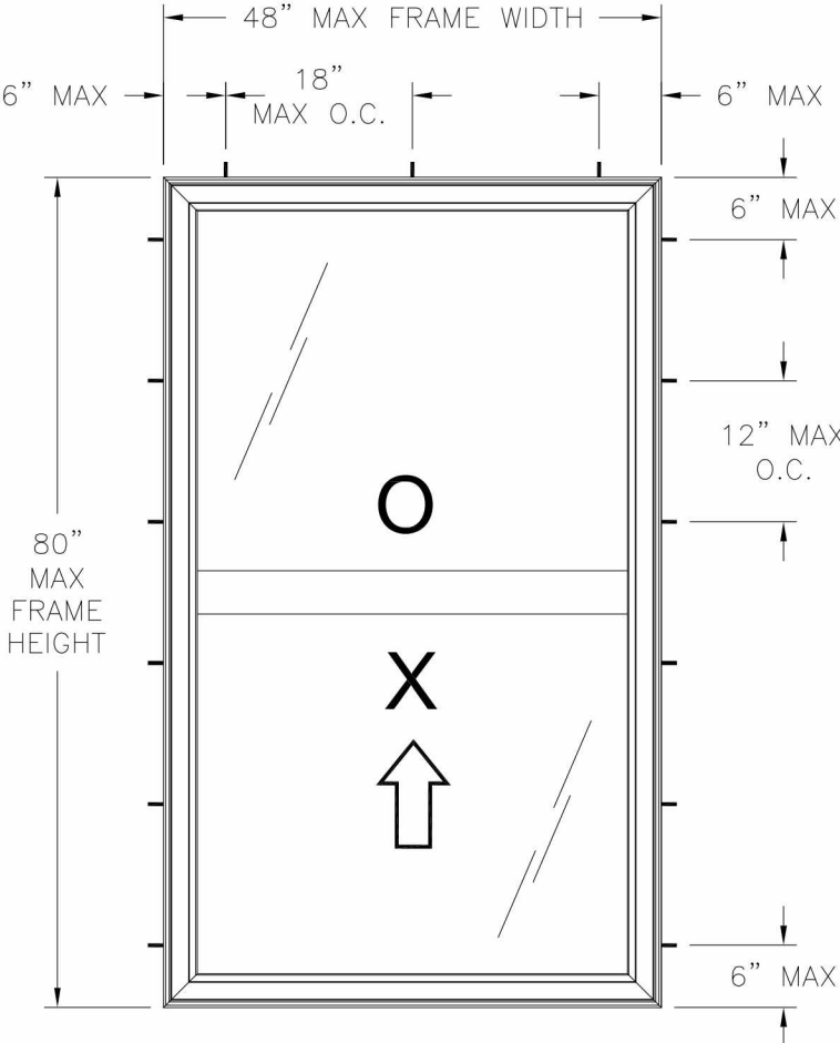
CAMBRIDGE SINGLE HUNG EXTERIOR VIEW FRAME INSTALLATION
