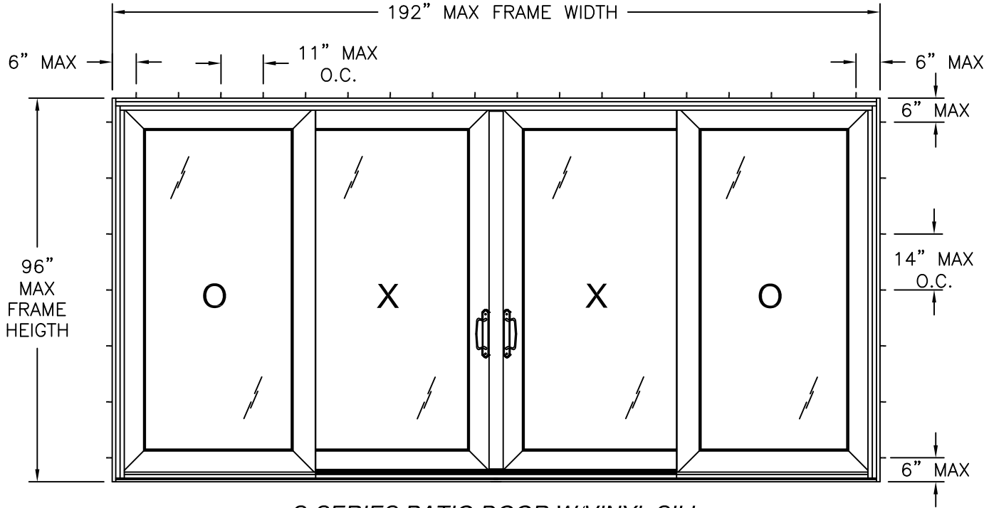
S-SERIES PATIO DOOR W/VINYL SILL EXTERIOR VIEW FRAME INSTALLATION
