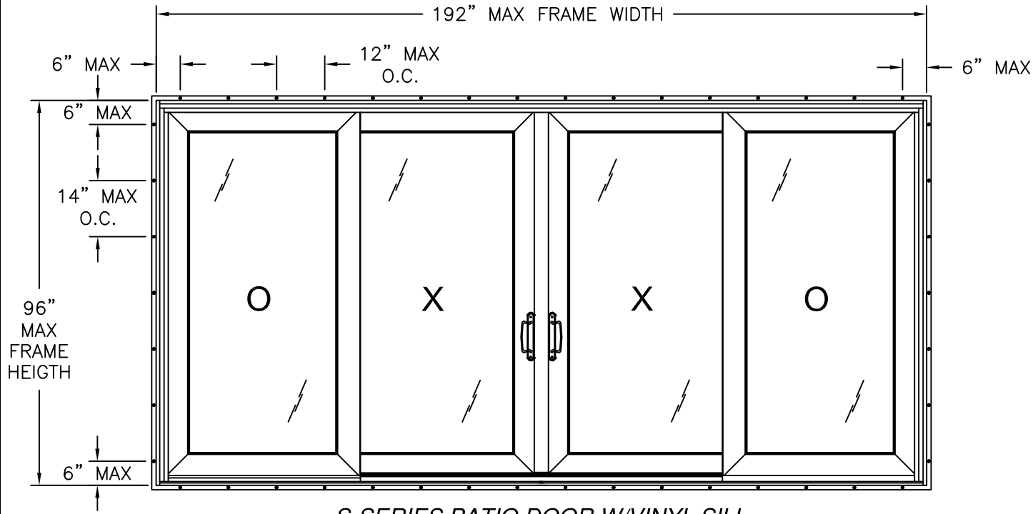
S-SERIES PATIO DOOR W/VINYL SILL EXTERIOR VIEW FIN INSTALLATION
