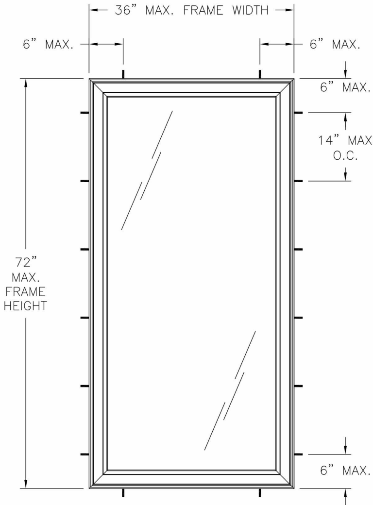
S-SERIES OCEANVIEW CASEMENT EXTERIOR VIEW FRAME INSTALLATION
