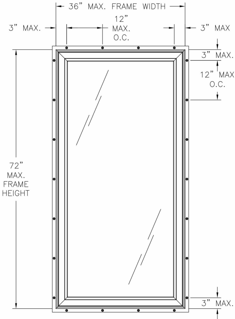
S-SERIES OCEANVIEW CASEMENT EXTERIOR VIEW FIN INSTALLATION
