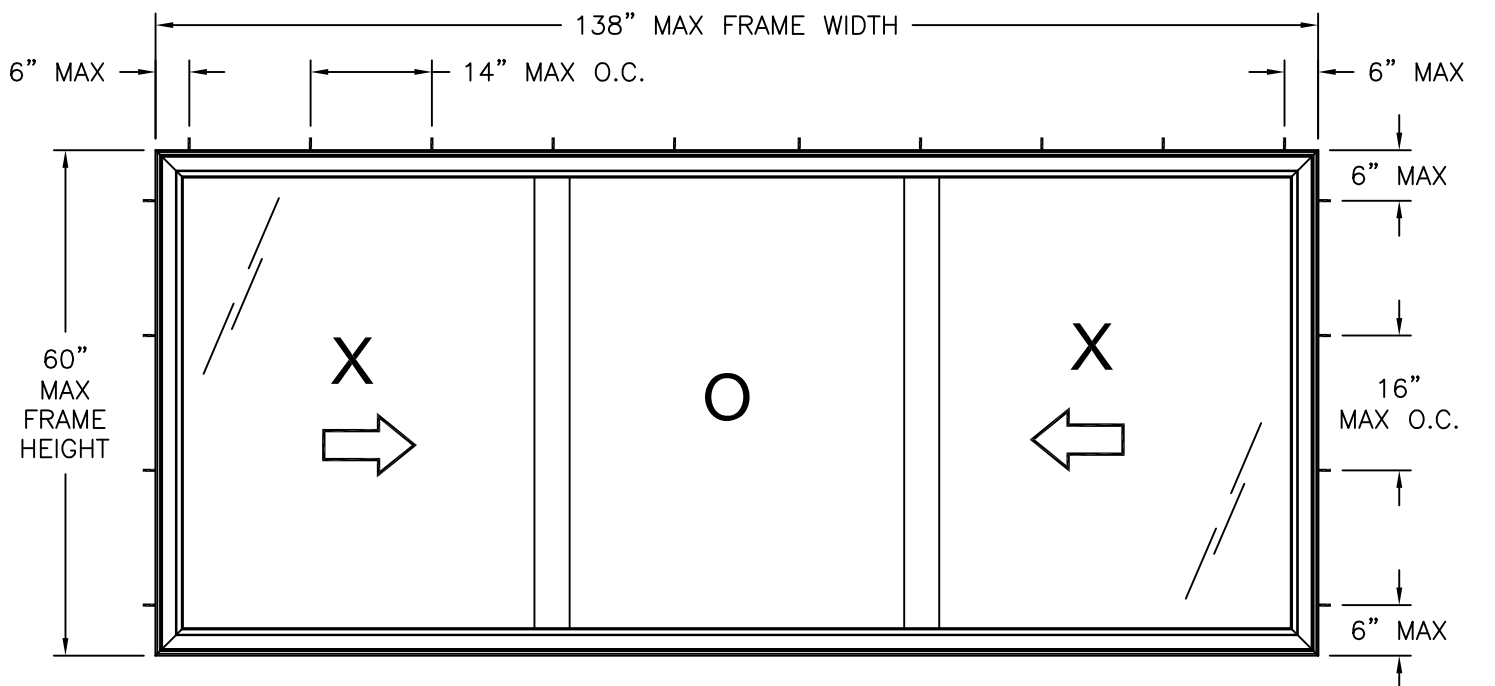
SIGNATURE/VIWINCO HORIZONTAL SLIDER XOX EXTERIOR VIEW FRAME INSTALLATION
